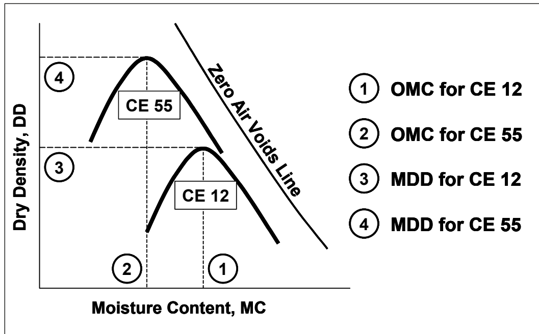
Figure 7. Typical behavior of moisture content-dry density Proctor curves.
