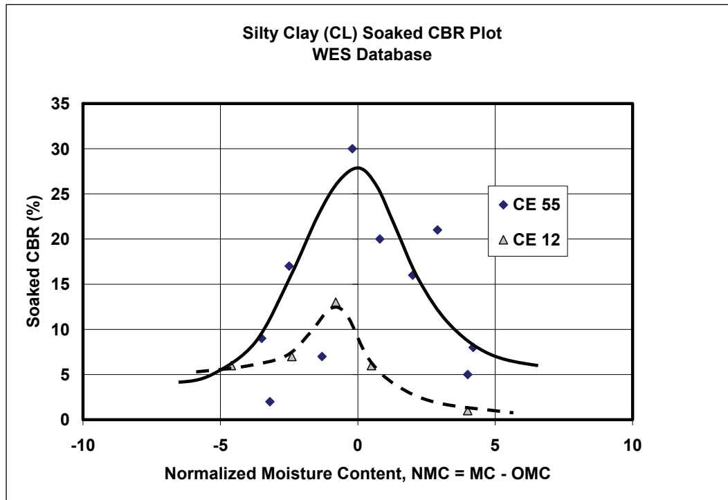
Figure 12. Response of soaked CBR in a normalized moisture content space.
