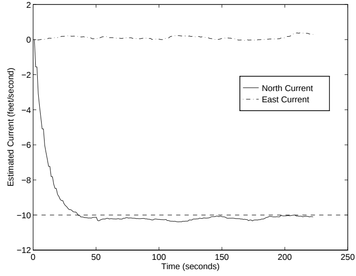
Figure 6: Estimated current for bench testing with water speed being set to 10.0 feet/second, K_1 = 0.1 , K_2 = 0.5 , K_3 = 2.0 and K_4 = 0.1 .
