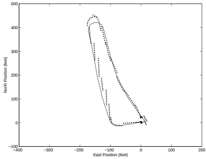
Figure 8: Position plot prior to compass calibration from ground vehicle testing with GPS update every 10 seconds.
