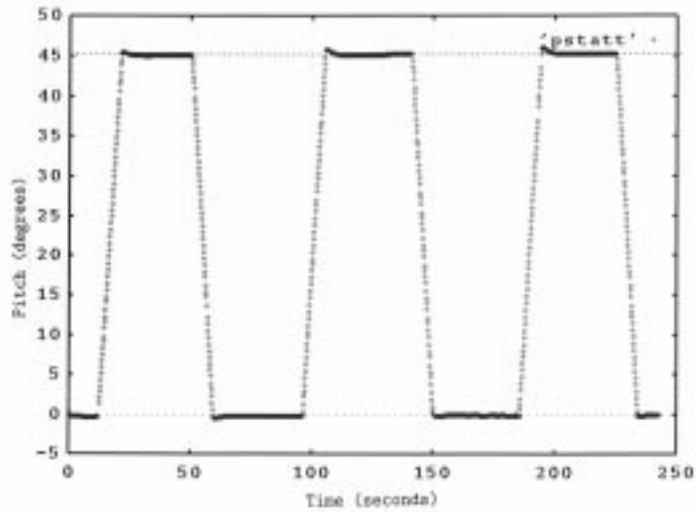
Figure 3: Forty-five degree pitch excursions at five degrees per second.
