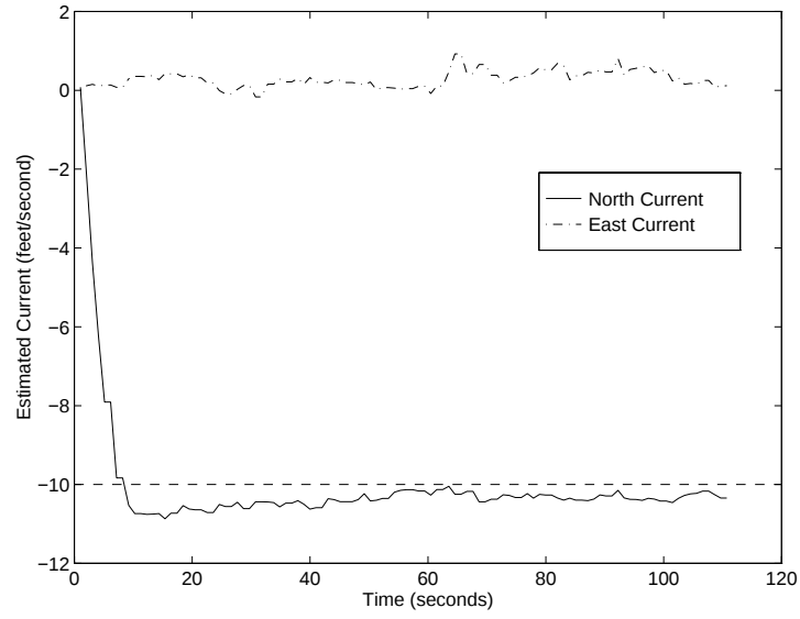
Figure 7: Estimated current for bench testing with water speed being set to 10.0 feet/second, K_1 = 0.1 , K_2 = 0.5 , K_3 = 0.5 and K_4 = 0.5 .
