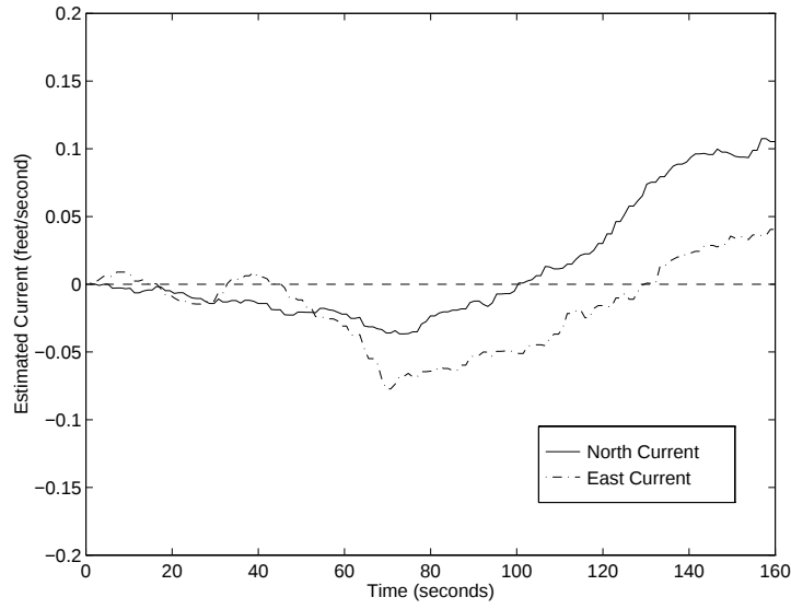
Figure 5: Estimated current for bench testing with water speed being set to zero, K_1 = 0.1 , K_2 = 0.5 , K_3 = 2.0 and K_4 = 0.01 .
