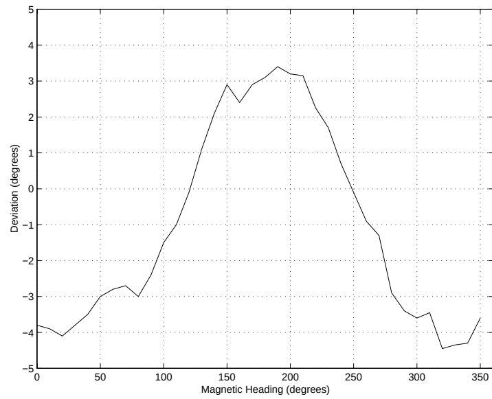
Figure 11: TCM-2 compass deviation.
