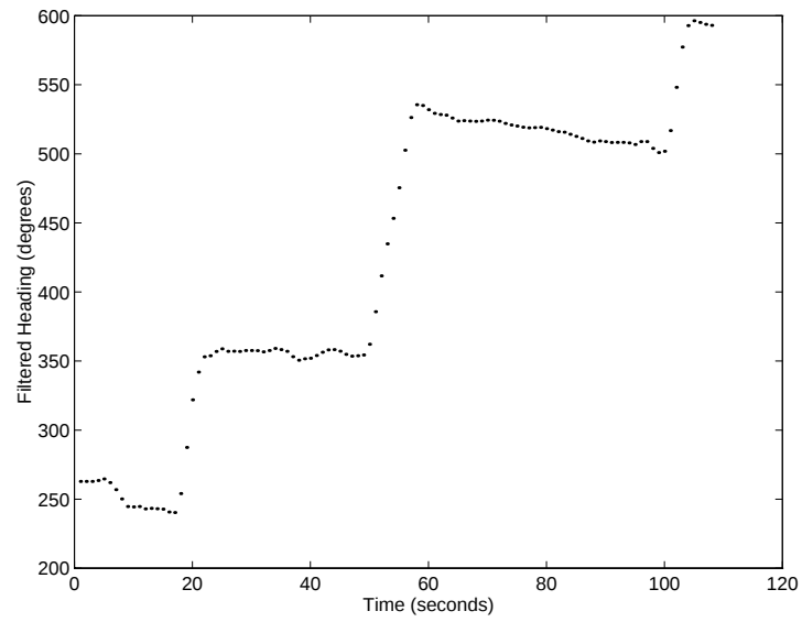
Figure 15: Filtered heading from ground vehicle testing.
