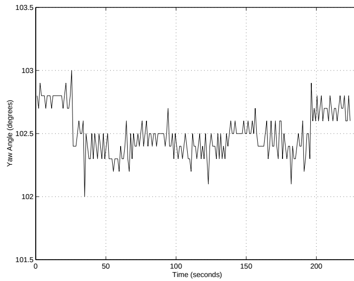
Figure 9: Effect of the golf cart motor on compass measurements.
