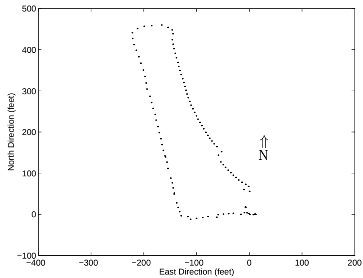
Figure 13: Position plot in one second increments from golf cart testing in the parking lot.
