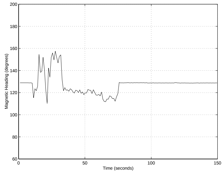
Figure 10: Effect of vibration on compass measurements.
