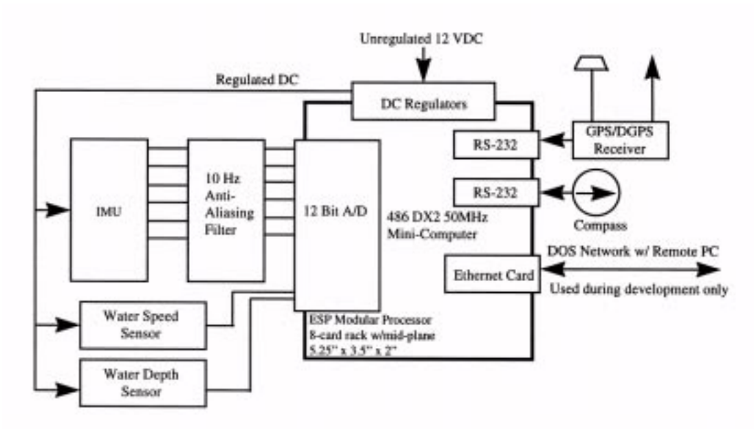
Figure 1: Block diagram of the new SANS hardware configuration.
