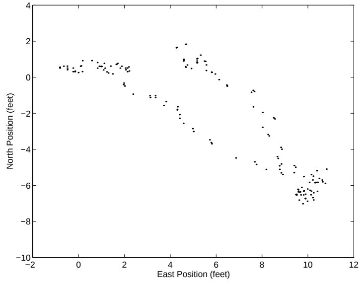
Figure 4: Position plot of bench testing with water speed being set to zero, K_1 = 0.1 , K_2 = 0.5 , K_3 = 2.0 and K_4 = 0.01 for a duration of 160 seconds.
