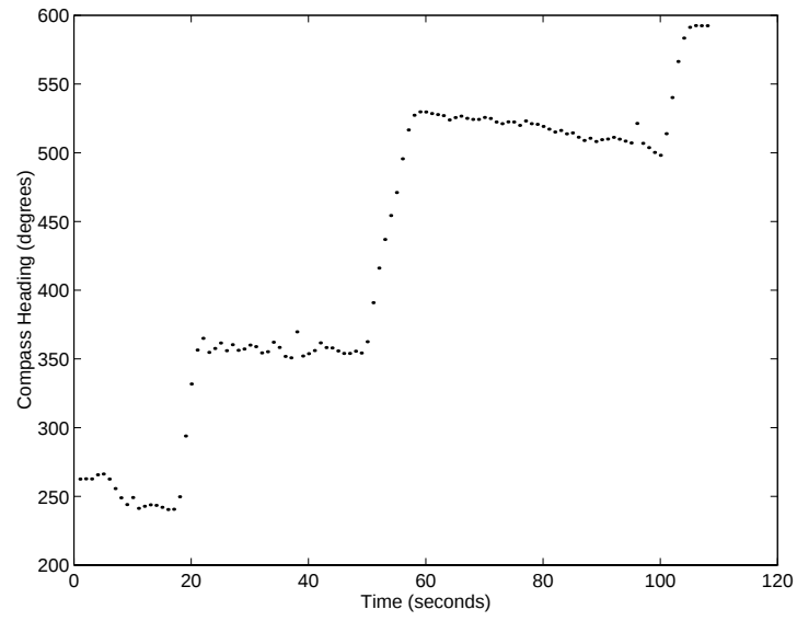
Figure 14: Compass heading from ground vehicle testing.
