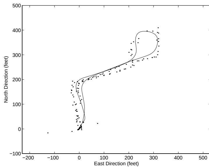
Figure 18: Ground vehicle test result with calibrated compass and bicycle wheel speed measurement. Dotted line: with GPS; solid line: without GPS.
