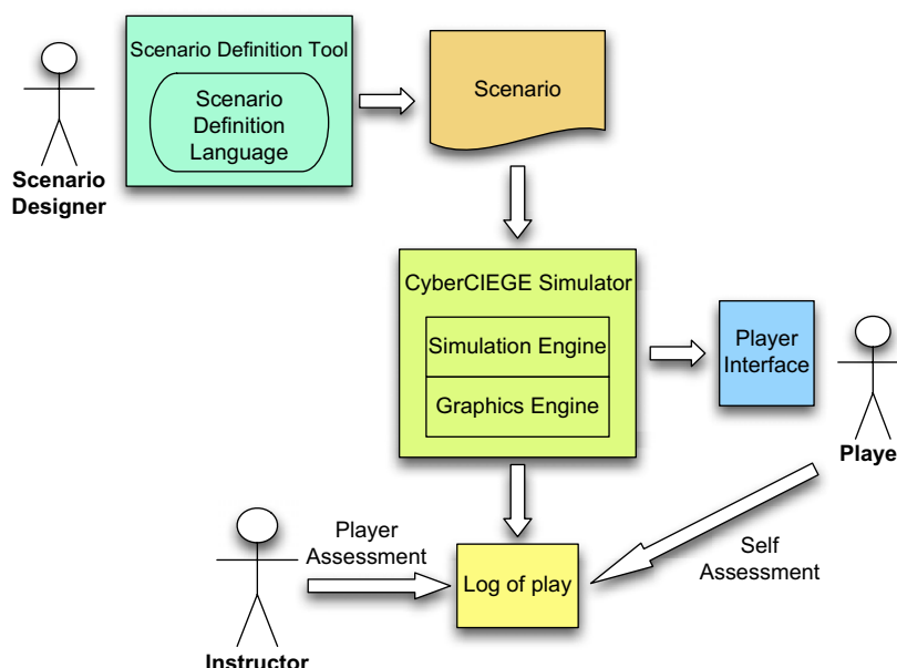
Fig. 1 – CyberCIEGE components.
