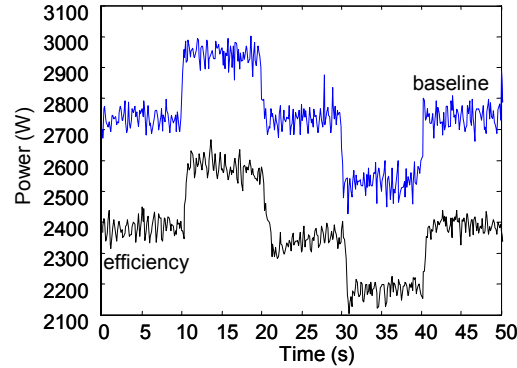
Figure 3. Improved efficiency for an earthmoving vehicle powertrain [14].
