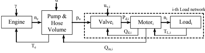
Figure 2: EVPS Schematic
