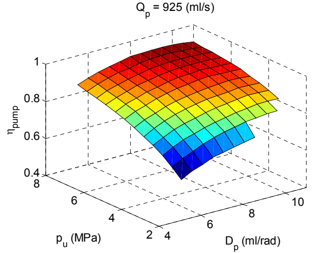
Figure 3: Steady-State Pump Map
