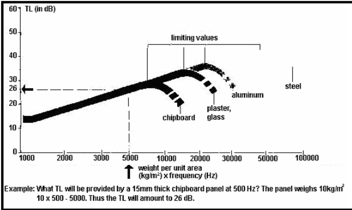
Figure 19: Transmission Loss for Different Materials
