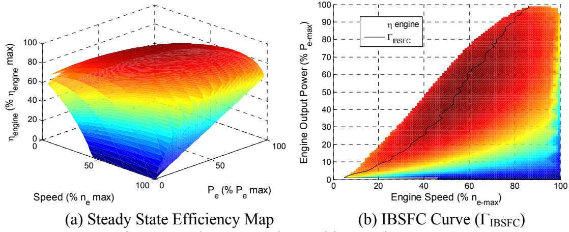
Figure 2. Unit Compression Ignition Engine Maps [11]
