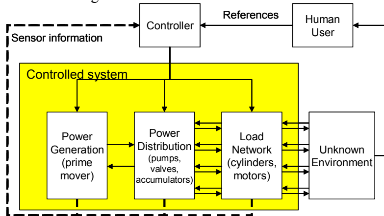
Figure 1. General framework for mobile energy management system with fluid power
