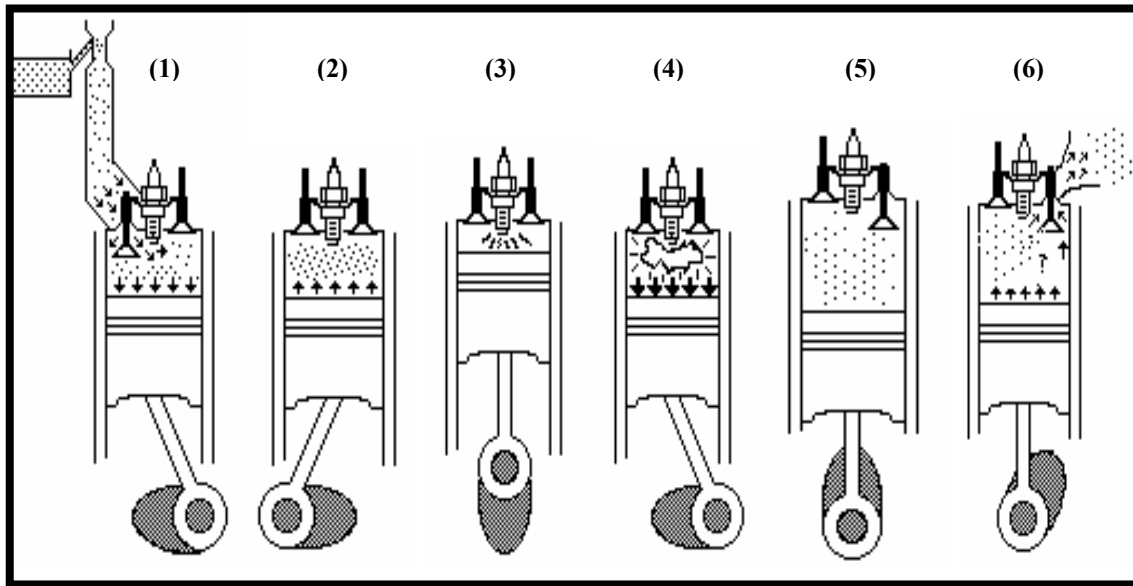
Figure 14: Diagrams Illustrating the Otto Cycle [29]
