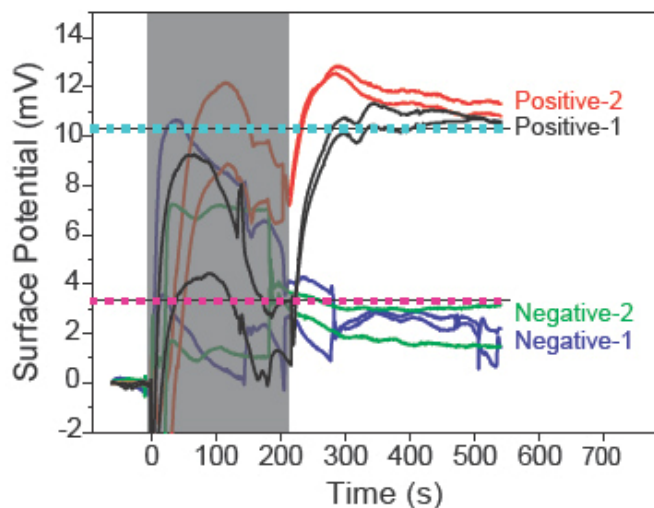
Figure 4: Integrated PCR and field-effect sensing of product. The sensor was functionalized, pressure was applied to flow the content of PCR channel over electronic sensors, after which valves were closed and measurement buffer flow was restored. The PCR channel was replenished with starting PCR reagent as its content was flowed into the sensing channel. The grey-out area indicated the period of PCR channel injection during which mechanical operations caused the sensor to lose its baseline value and drift temporarily. The higher and lower dotted segments are arbitrarily defined threshold levels for positive and negative signals, respectively.
