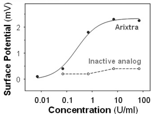
Figure 6: Dose-response curve of the AT-III-sensor for heparin-based pentasaccharide drug fondaparinux (●) and 6-O desulfated fondaparinux (○), which is known to exhibit low binding affinity for AT-III. Data points for fondaparinux are fit with a Langmuir isotherm (solid line), and those for and 6-O desulfated fondaparinux are connected with a dashed line. Note that 0.2 U/mL ~ 1mg/ml ~ 50 nM
