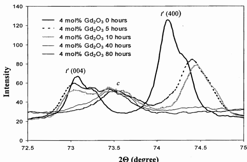
Figure 7. X-ray diffraction pattern of the {400} region of plasma-sprayed \text{ZrO}_2 -4 mol% \text{Gd}_2\text{O}_3 powder after heat treatment for 0, 5, 10, 40, and 80 hours at 1400 °C.
