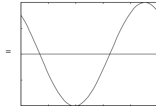
Expected Response
