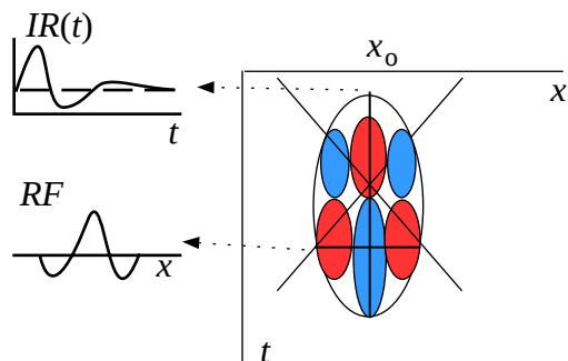
Spectro-Temporal Domain
