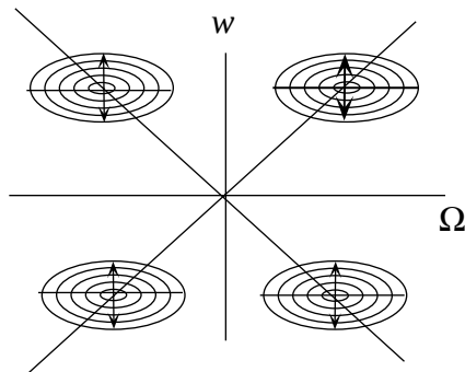
Fourier Domain
