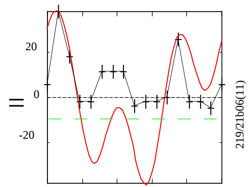
Response
