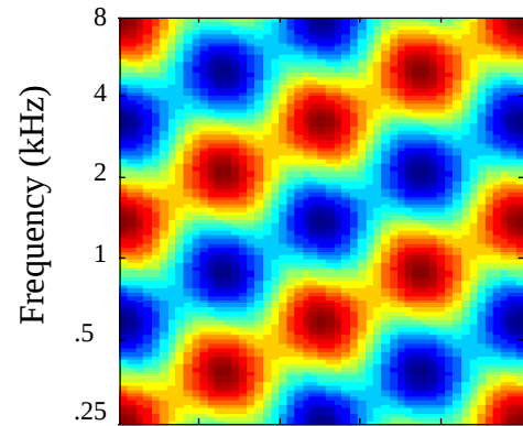
Stimulus Spectrogram
