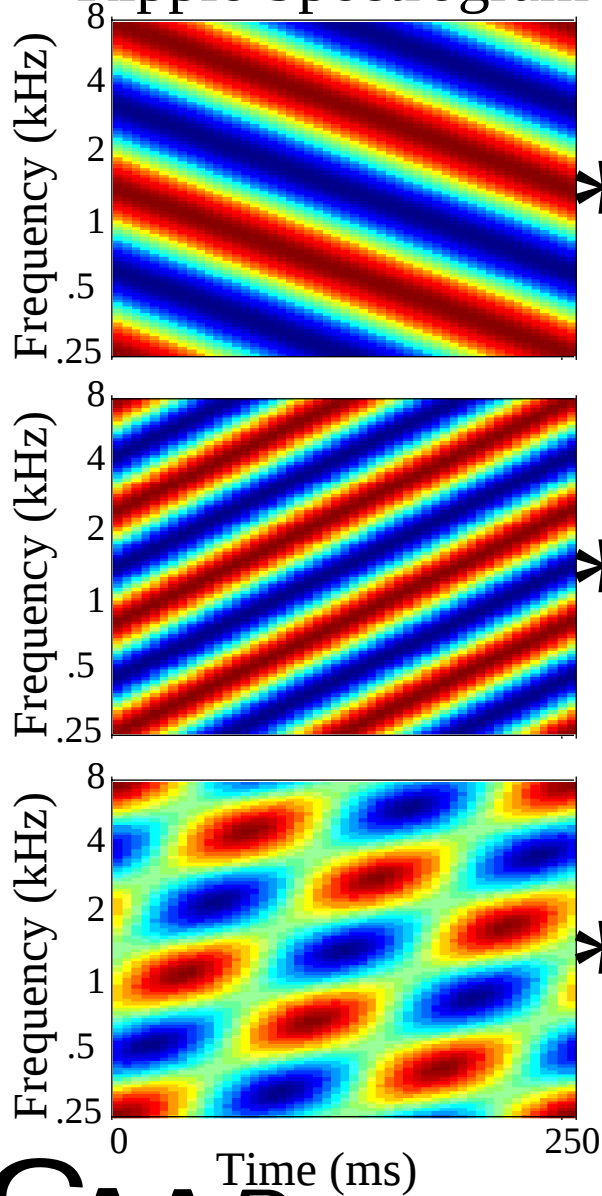
Ripple Spectrogram
