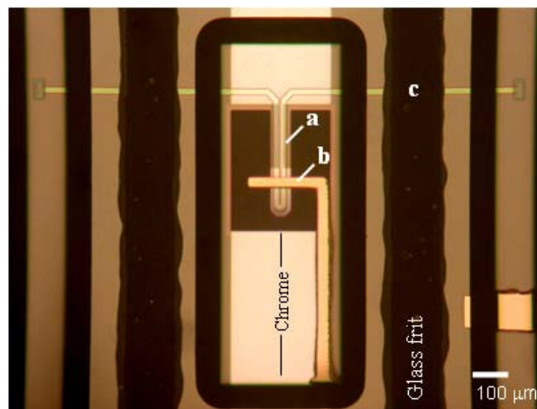
Figure 6: Optical micrograph of a packaged cantilever resonator. The 300 \mu\text{m} long beam contains a 1 \times 20 \mu\text{m} microfluidic channel (a). An electrode on the glass surface above the cantilever enables electrostatic actuation (b). Glass frit conforms to the surface topography and does not collapse the thin channel in location (c) during bonding.
