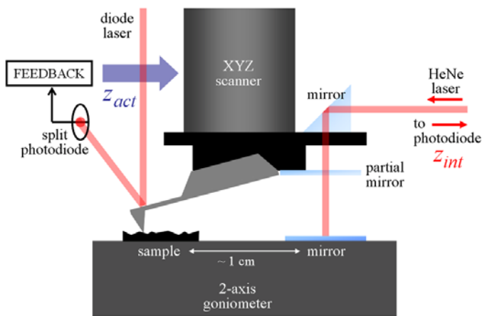
Figure 3: Experimental schematic. Z_{act} (actuator) is the signal that is used for conventional scanning probe microscopy and includes a superposition of topography and mechanical disturbances. However, Z_{int} (interferometer) reveals only topography and suppresses the mechanical disturbances.
