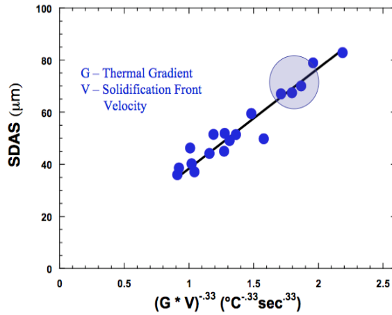
Figure 13: Measured Secondary Dendrite Arm spacing plotted as a function of the product of (G*V)^{-.33}
