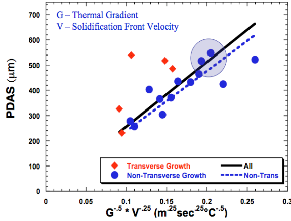
Figure 12: Measured Primary Dendrite Arm spacing plotted as a function of the product of G^{-.5} * V^{-.25}
