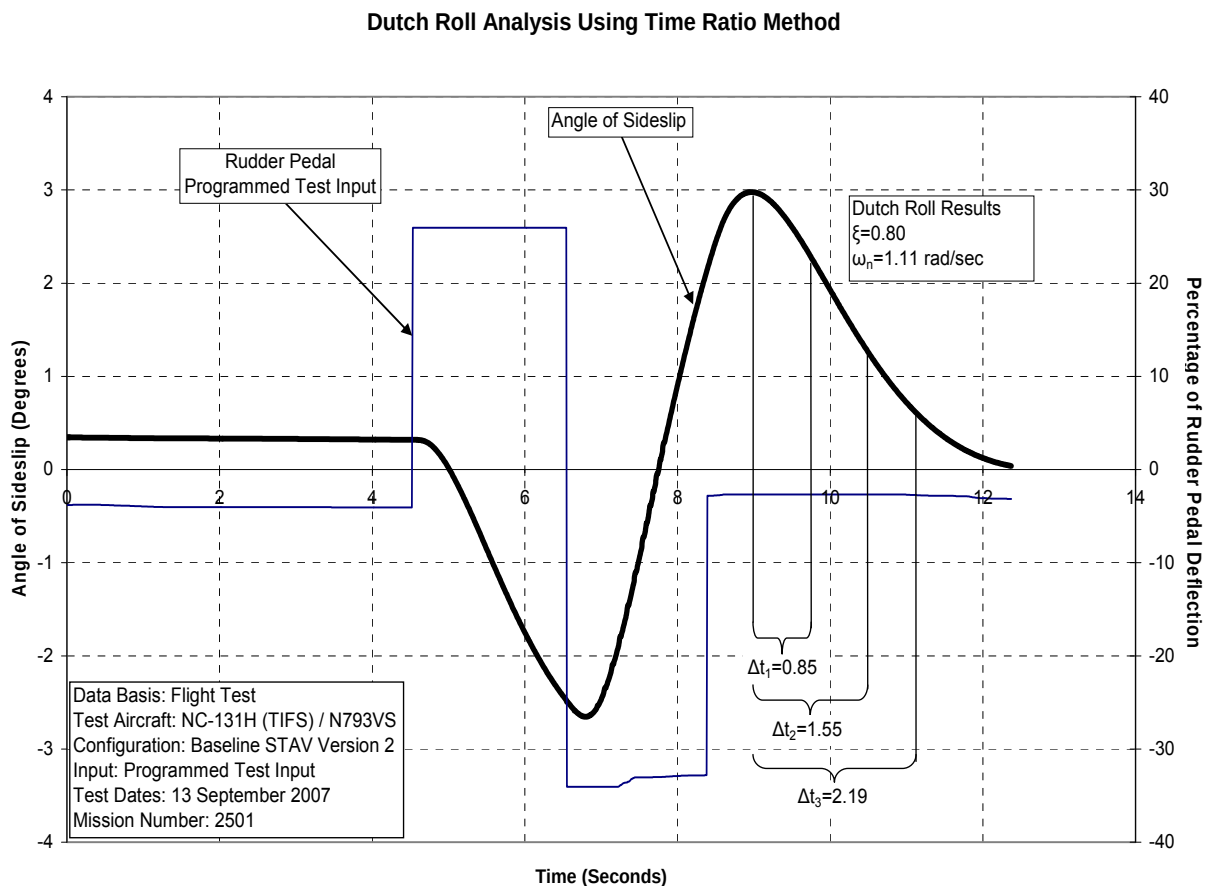
Figure 46 – Dutch Roll Analysis Using Time Ratio Method
