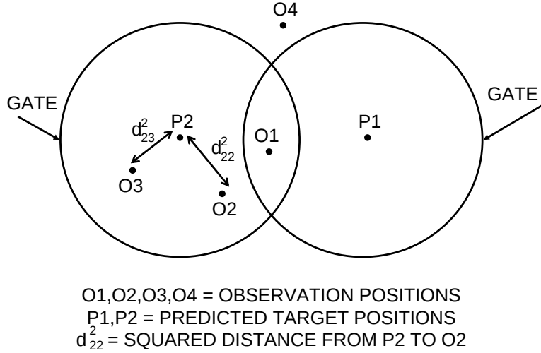
Figure 2.12: This data association example consists of two closely spaced targets (P1 and P2) and four observations (O1...O4). The potential pairings are P1-O1, P2-O1, P2-O2, and P2-O3. Since O1 is the only observation within the gate of track P1, it will likely be associated with P1, whereas P2 will be associated with either O2 or O3, which depends on the results of the association algorithm.
