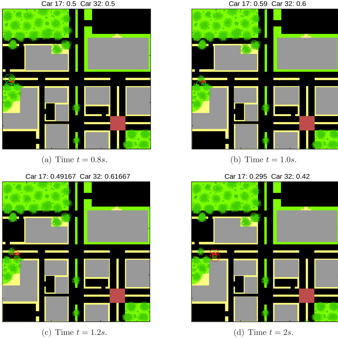
Figure 4.4: Kinematic-only tracking for configuration 1 (Part A). This configuration consists of a class ID 17 (red 1 ) and a class ID 32 (green) vehicle. Both vehicles start out heading east. The tracker initiates each track using the class ID state of the nearest vehicle (a). Because of tree occlusions, the tracker deletes the class ID 17 (red 1 ) track (b) and swaps the class ID 32 (green) track to the class ID 17 (red 1 ) vehicle (c). After the vehicles pass the trees, the tracker initiates a track and assigns it the class ID 17 (red 1 ), which is the nearest vehicle. The tracker updates the class ID 17 (red 1 ) track using the kinematic measurements of class ID 32 (green) vehicle.
