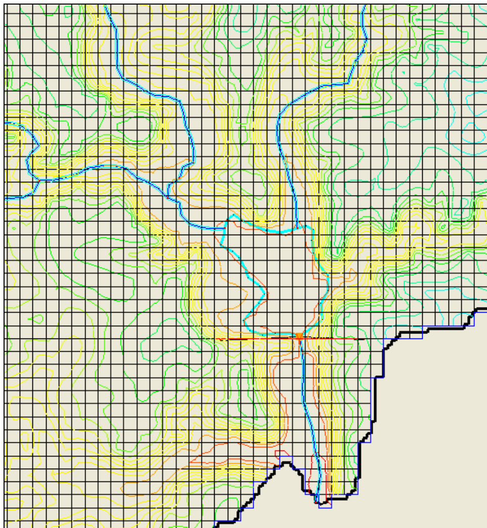
Figure 2. Reservoir representation in GSSHA stream network and 2-D grid.
