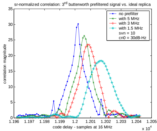
Figure 19 – Bandwidth on Square-Root Normalized Correlation (Ideal Replica)
