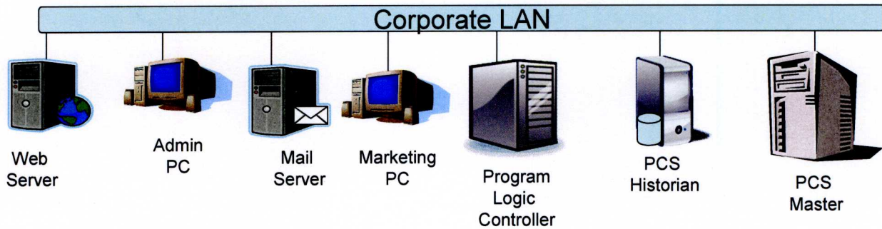
Figure 3. Integrated PCS
