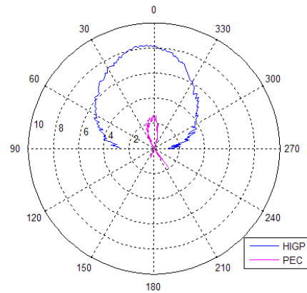
Figure 64: 11 by 11 Square Patch HIGP with 0.4 \lambda_{12\text{GHz}} -Dipole Horizontal Measurement
