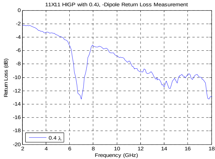
Figure 61: 11 by 11 HIGP with 0.4\lambda_{12\text{GHz}} -Dipole Return Loss Result
