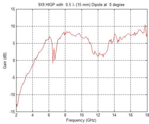
Figure 55: 9 by 9 Square Patch HIGP with 0.5 \lambda_{10\text{GHz}} -Dipole Horizontal Measurement
