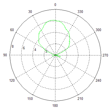
Figure 72. Log-periodic Antenna Free Space Measurement
