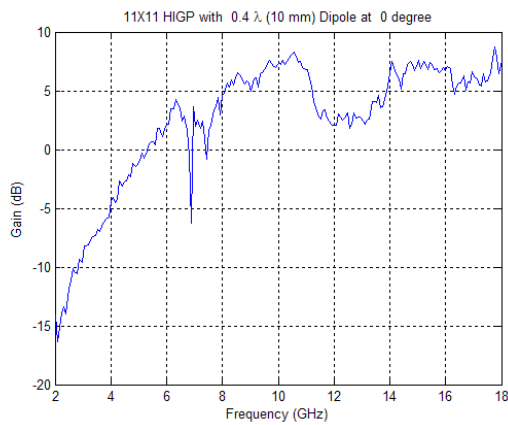
Figure 64: 11 by 11 Square Patch HIGP with 0.4 \lambda_{12\text{GHz}} -Dipole Horizontal Measurement
