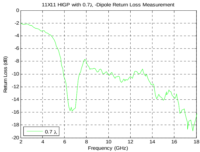
Figure 63: 11 by 11 HIGP with 0.7 \lambda_{12\text{GHz}} -Dipole Return Loss Result
