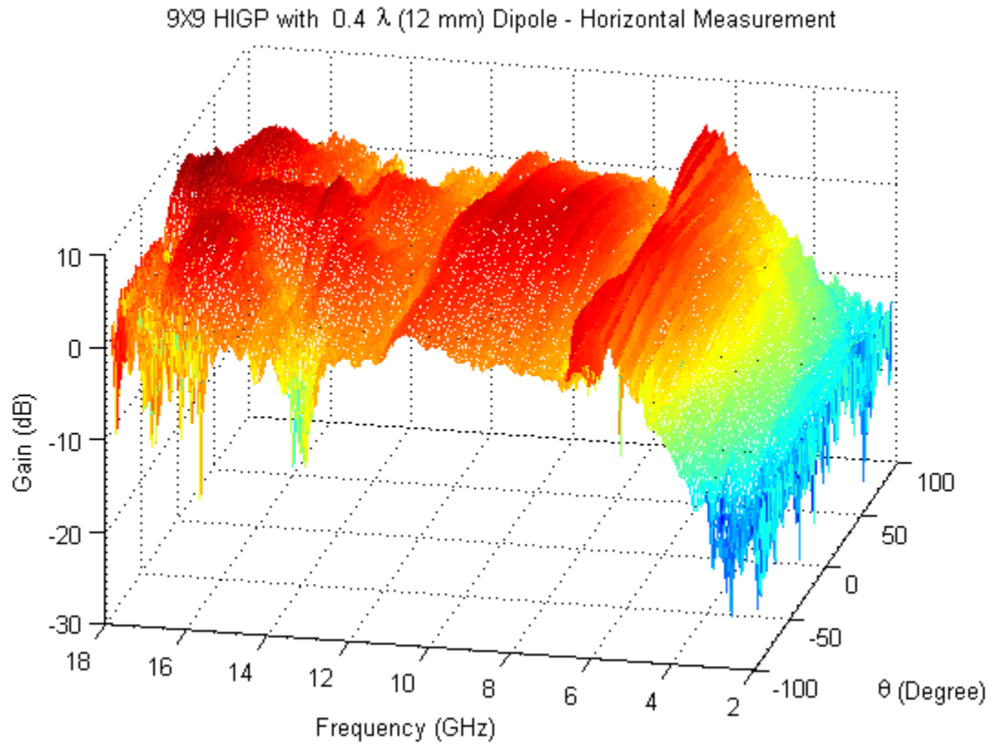
a) 9 by 9 0.4 \lambda_{10\text{GHz}} Dipole Antenna Pattern
