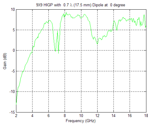
b) Gain Performance
