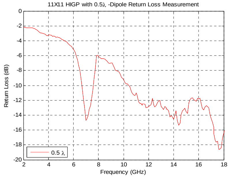
Figure 62: 11 by 11 HIGP with 0.5 \lambda_{12\text{GHz}} -Dipole Return Loss Result
