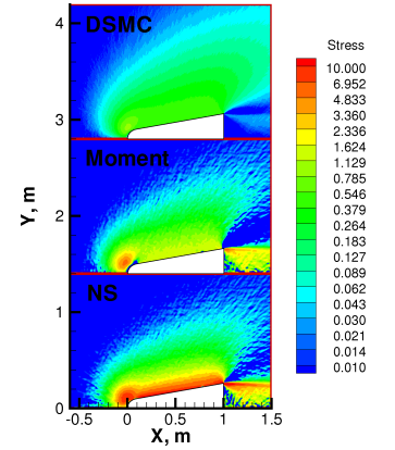
FIGURE 10. Shear stress contours, Kn = 10^{-1} : DSMC, Anisotropic, NS
