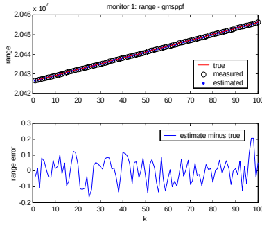
Figure 19 – Monitor 1's Measurements for GMSPPF
