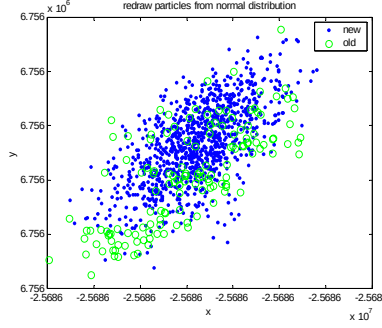
Figure 31 - Particle Redrawing with Estimated Distribution
