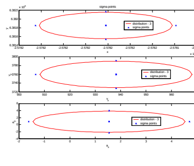
Figure 25 - Sigma-Points Selected for Position, Velocity, and Acceleration
