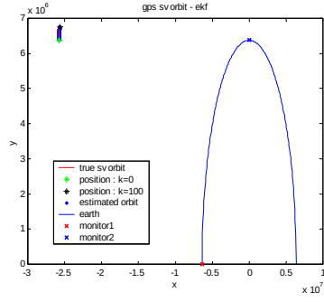
Figure 6 - Orbit Estimated by EKF
