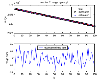
Figure 20 – Monitor 2's Measurements for GMSPPF
