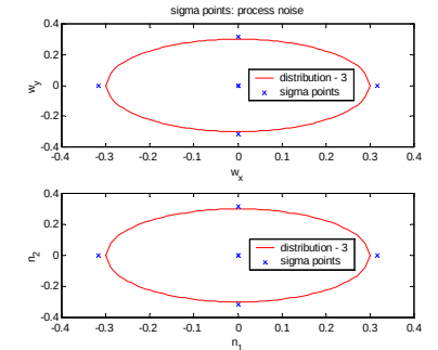
Figure 26 - Sigma Points Selected for Process Noise and Measurement Noise
