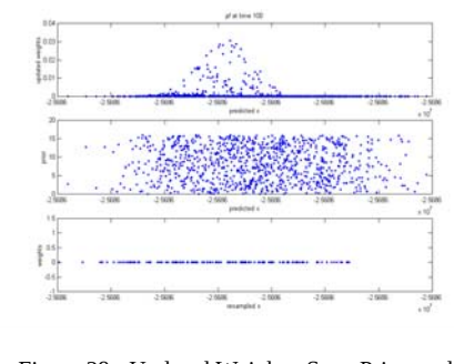
Figure 29 - Updated Weights, State Prior, and Weights After Resampling
