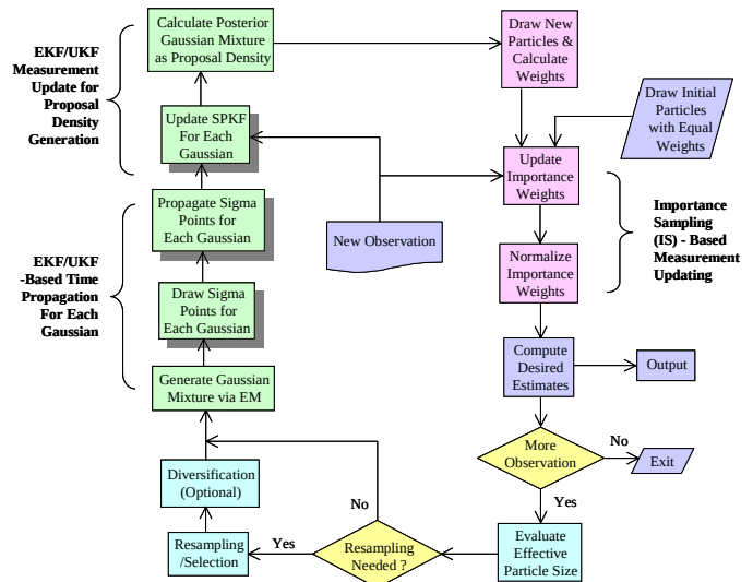
Figure 3 – Block Diagram of Hybrid Kalman Particle Filter
