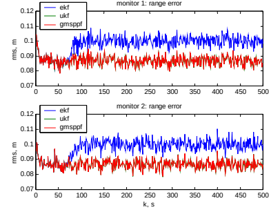
Figure 32 - RMS Values for Measurement Residuals
