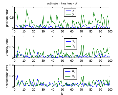
Figure 17 - State Estimation Errors for PF
