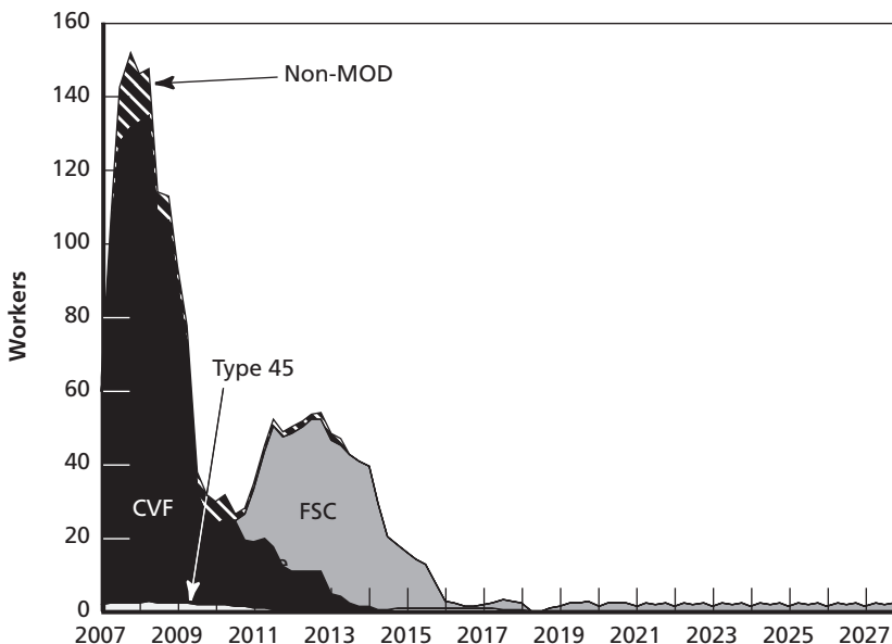
Figure 6.3 Technical Labour Demand for Detailed Designer Electrical and Control Skill, Complex Surface Ship Programmes
