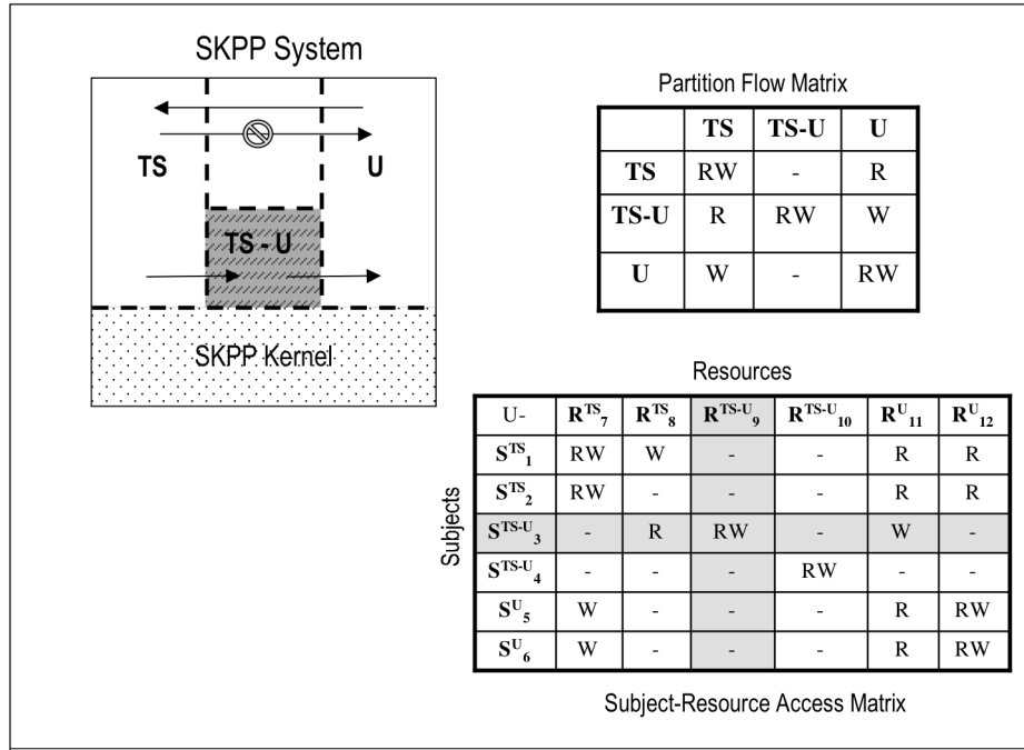
Figure 2: Kernel-based Strictly-Controlled Interference
