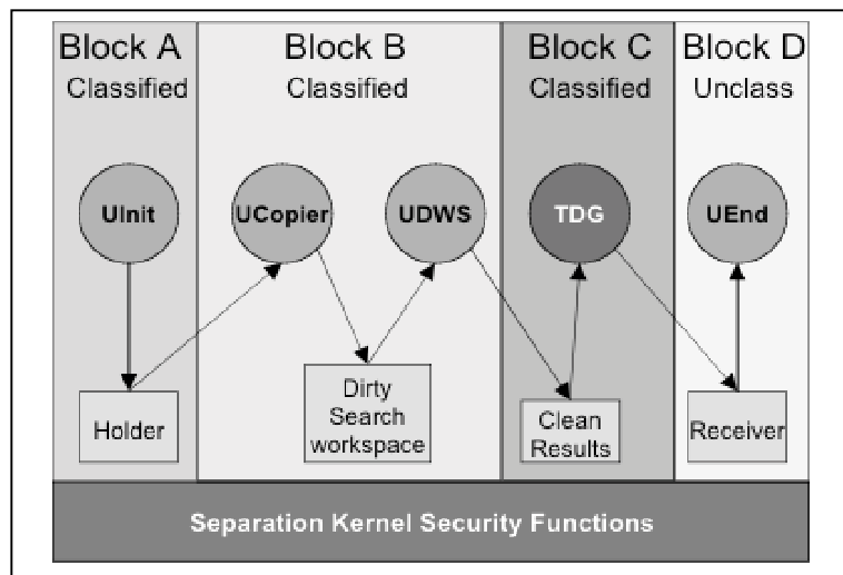
Figure 3: Trusted Downgrader. Dark areas with white text are trusted.
