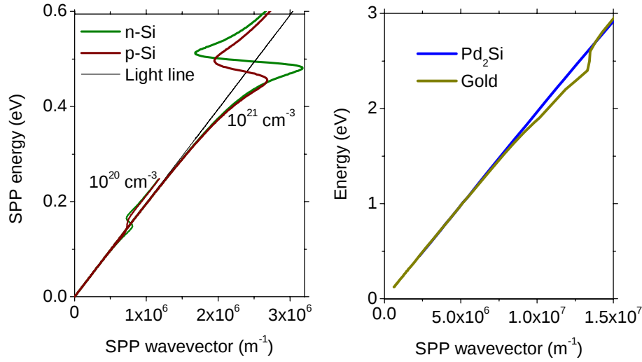
Fig. 3. (left) SPP dispersion curves for doped silicon; (right) SPP dispersion curves for gold and Pd 2 Si.
