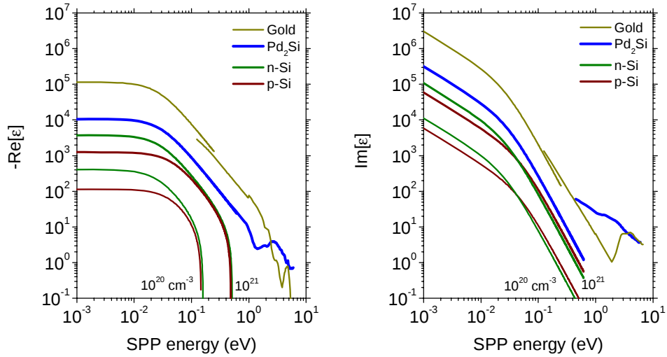
Fig. 2. Permittivities -\epsilon'(\omega) and \epsilon''(\omega) of doped-Si and \text{Pd}_2\text{Si} compared with those of gold.
