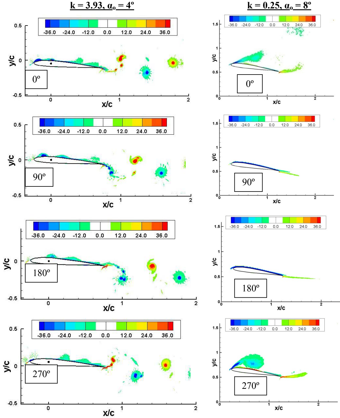
Figure 41: Vorticity ( \omega_z/U_\infty/c ) contours examining reduced frequency effects for pure-plunge for k = 3.93 and k = 0.25 , \text{Re} = 60 \times 10^3 .
