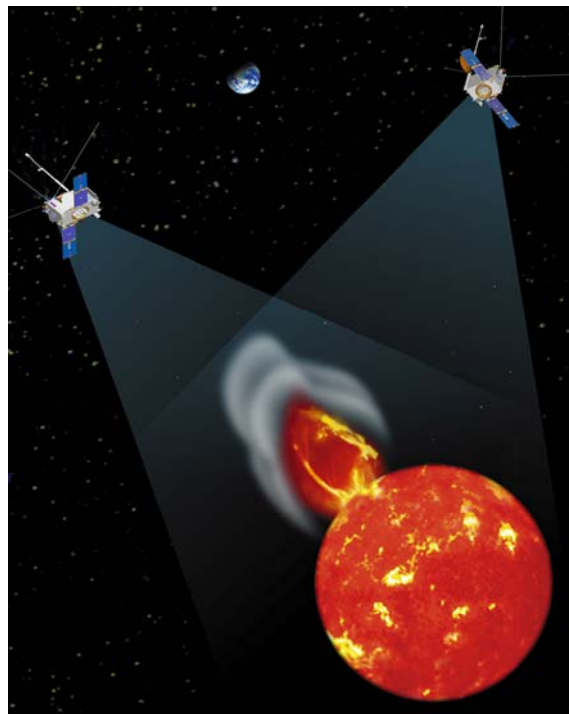
Figure 5. STEREO
