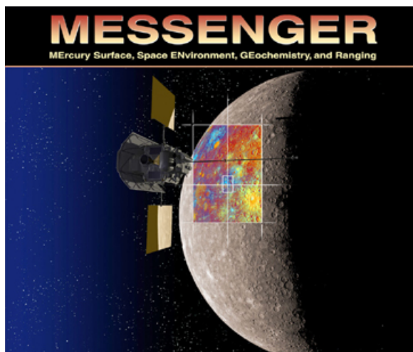
Figure 1. MESSENGER
