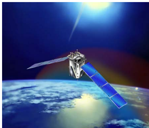
Figure 2. TIMED
