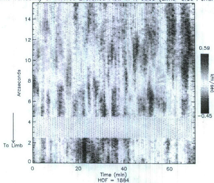
Time Variability of Inverse Evershed Flow in H 6563 (Limb-side Penumbra)
