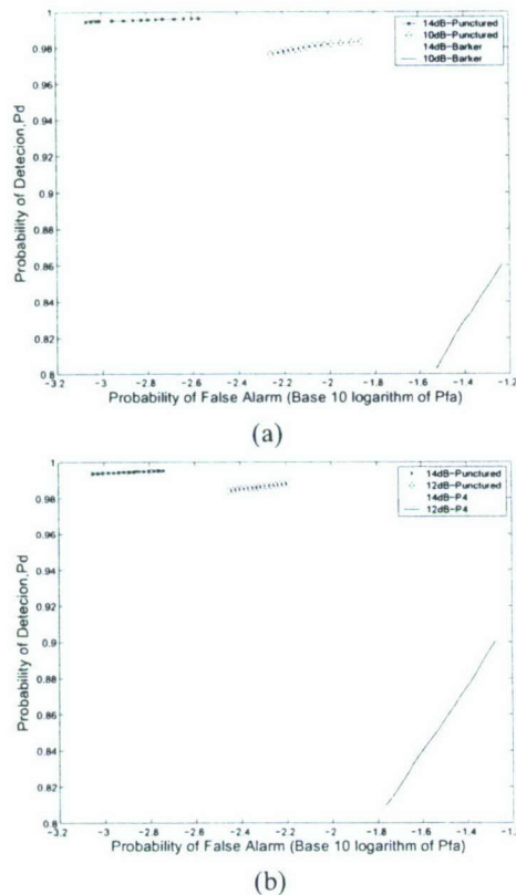
Fig. 7. Probability of detection versus probability of false alarm of the coherent receiver (No time delay, Doppler shift less than 1): (a) 13-length Punctured binary sequence-pair VS. 13-length Barker code (b) 31-length Punctured binary sequence-pair VS. 31-length P4 code
