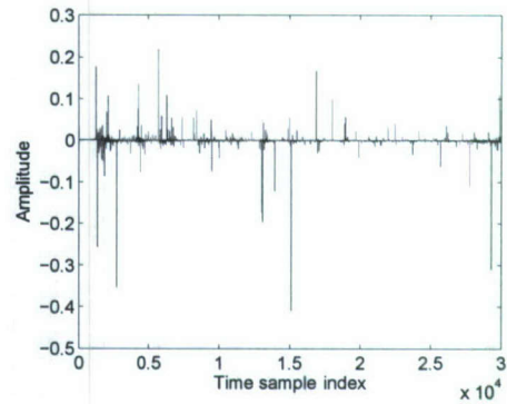
Fig. 7. 200MHz Channel
