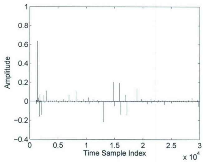
Figure 8: 400MHz Channel
