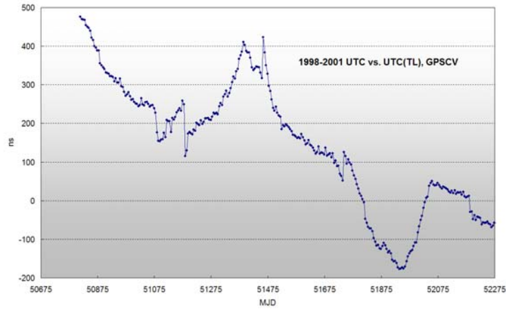
Figure 9. UTC – TA (TL), before 2002.
