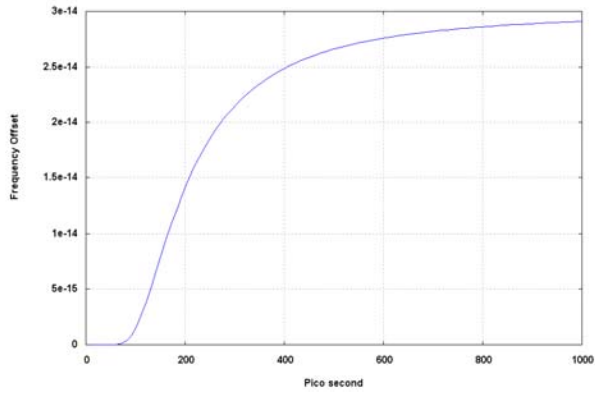
Figure 4. The pattern of control law: 3 \times 10^{-14} \cdot \exp(-3/(\alpha \cdot 2)) .
