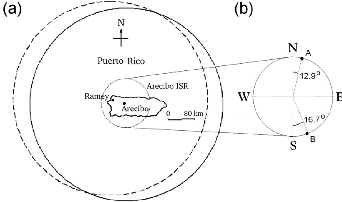
Figure 5. (a) Map of Puerto Rico showing the field of view of Ramey ionosonde (dashed line) and Arecibo ionosonde (solid line), at an altitude of 300 km. The dotted line shows the trace cross-section of Arecibo ISR when the beam is rotating and at a maximum angle from the zenith. (b) Arecibo ISR beam trace cross-section.
