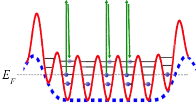
Figure 7. Scheme for preparing a near-zero-temperature Fermi gas. Initially, atoms at a density greater than 1 atom per lattice site and a temperature T \sim 0.1 T_F are loaded into an optical lattice. The occupation number for states in the first band is very close to unity, whereas the occupation number for states near the Fermi surface in the second band can be less than unity. A near-zero-entropy state is prepared by selectively removing atoms in the second band from the lattice potential.
