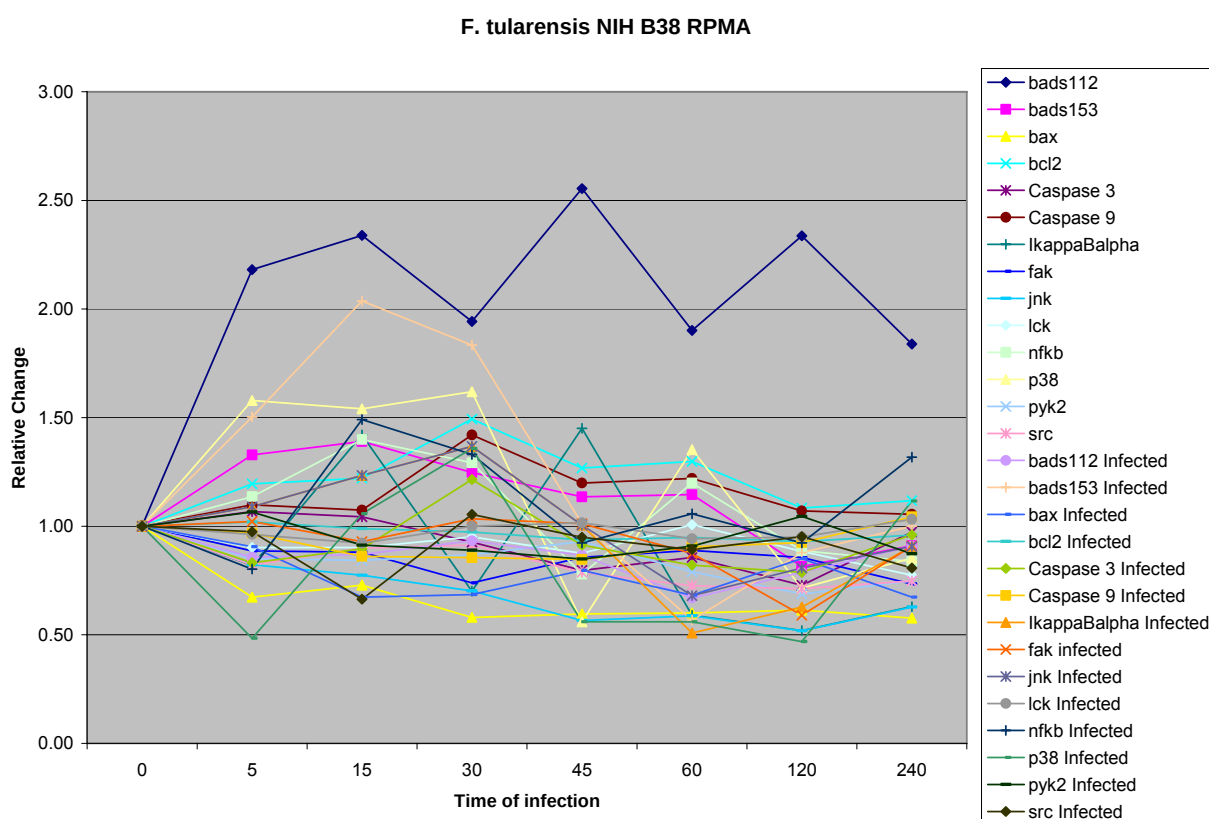
Figure 1.5B: Relative Changes in Activation of Francisella tularensis NIH B38 infected vs. uninfected J774A.1 macrophages. In this figure, the infected numbers were divided by the uninfected numbers to illustrate the fold change in signal for each antibody. This representation of fold-change simplifies the data set and allows up to observe which molecules are significantly up-regulated (greater than 1.5) or down-regulated (less than 0.5) following infection by Francisella B38.
