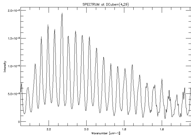
Figure 10a: reconstructed spectrum (wavenumber)
