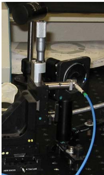
Figure 6: Mirror and fiber optic waveguide at exit slit of monochromator
