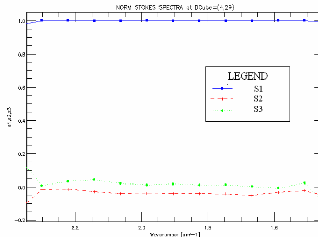
Figure 10b: normalized reconstructed Stokes spectra
