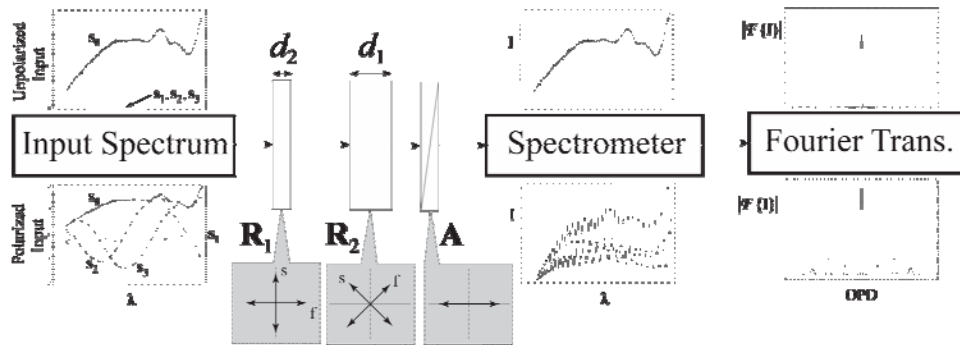
Figure 3: Schematic diagram of a channeled spectropolarimeter.
