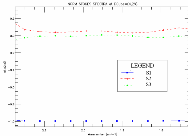
Figure 11b: normalized reconstructed Stokes spectra
