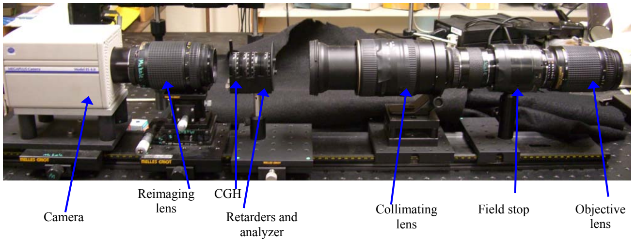
Figure 5: picture of CTIS instrument with labels showing individual elements
