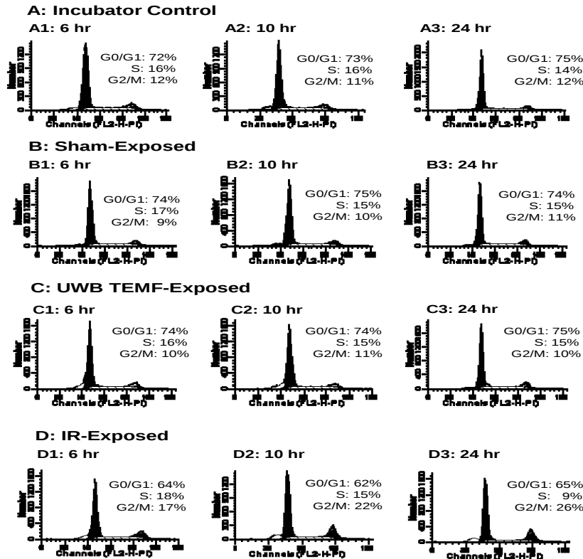
Figure 1: Cell cycle distribution after UWB TEMF exposures in 244B human lymphoblastoid cells. A-Incubator control: A1 (at 6 hour), A2 (at 10 hour), A3 (at 24 hour). B-Sham-exposed: B1 (at 6 hour), B2 (at 10 hour), B3 (at 24 hour). C-UWB TEMF-exposed: C1 (at 6 hour), C2 (at 10 hour), C3 (at 24 hour). D: Ionizing radiation (IR)-exposed (5 Gy): D1 (at 6 hour), D2 (at 10 hour), and D3 (at 24 hour). Left peak, middle plateau, and right peak represent cells in G0/G1, S, and G2/M phases of the cell cycle, respectively.
