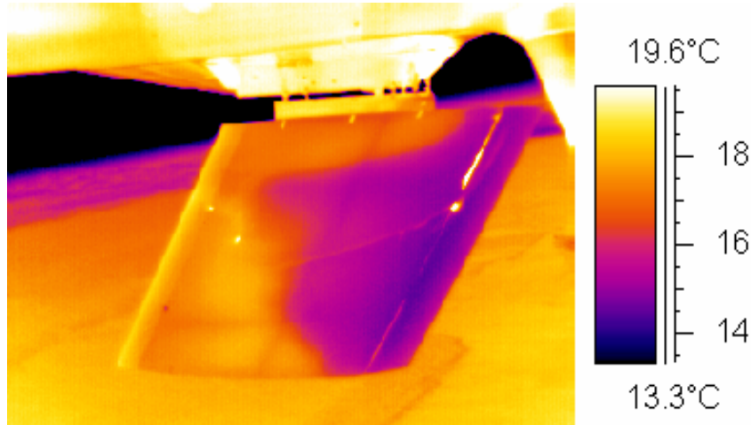
Figure 4. 180 KTAS, AoA = -4 , Re_c = 8.0 \times 10^6 , White painted LE, DRE x 2 placed at 1\% x/c at inboard pressure row, and 1.3\% x/c at outboard pressure row, d = 1\text{ mm} , \lambda = 2.25\text{ mm} , transition moved to 60\% x/c
