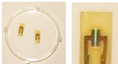
Figure 6. Photo of dodecylamine-mediated thin film assembly of Cu nanoparticles capped with oleyl amines applied at gap of Interdigitated Microelectrode (IME).
