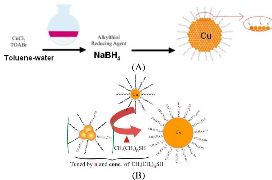
Scheme 3. The general schemes illustrating the two-phase synthesis of thiolate-capped Cu nanoparticles (TOABr: tetraoctylammonium bromide) (A) and the subsequent thermal processing to form larger-sized and shaped nanoparticles (B).
