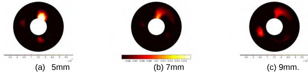
Figure 11. Experimental results for a 7.8mm blob of ~3 \times contrast in a 0.5% Intralipid solution. (a) Target depth of 5mm. (b) Target depth of 7mm. (c) target depth of 9mm.
