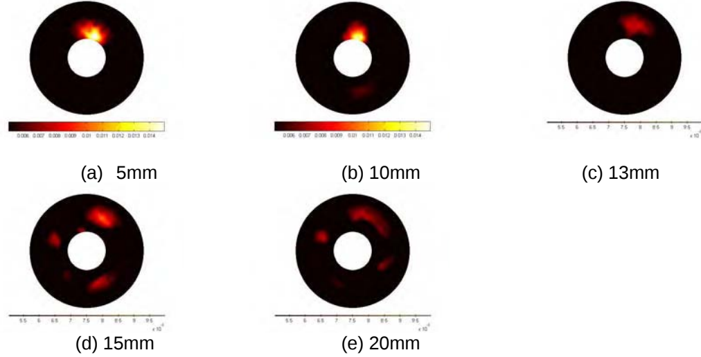
Figure 10. Experimental results for an 8mm blob of black absorbing rod in a 0.5% Intralipid solution. (a) Target depth of 5mm. (b) Target depth of 10mm. (c) Target depth of 13mm. (d) Target depth of 15mm. (e) Target depth of 20mm.
