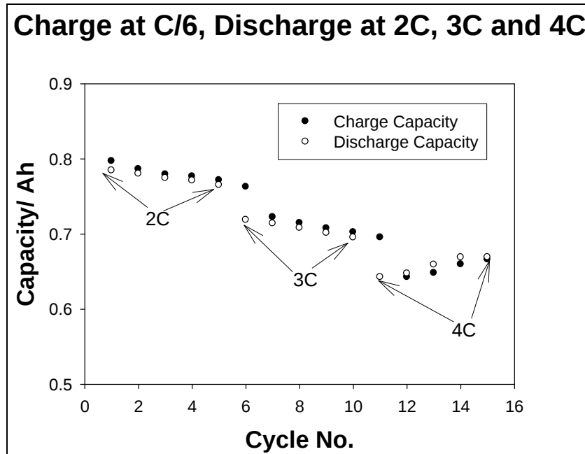
Figure 7. Effect of discharge rate on Nexlion cell cycling.
