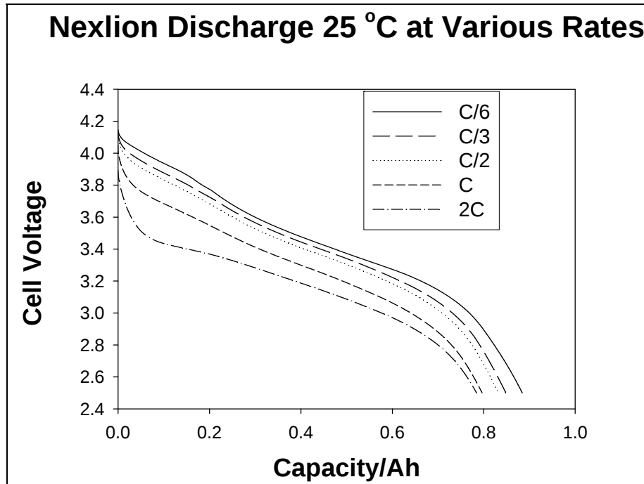
Figure 6. Discharge of Nexlion cell at various rates.
