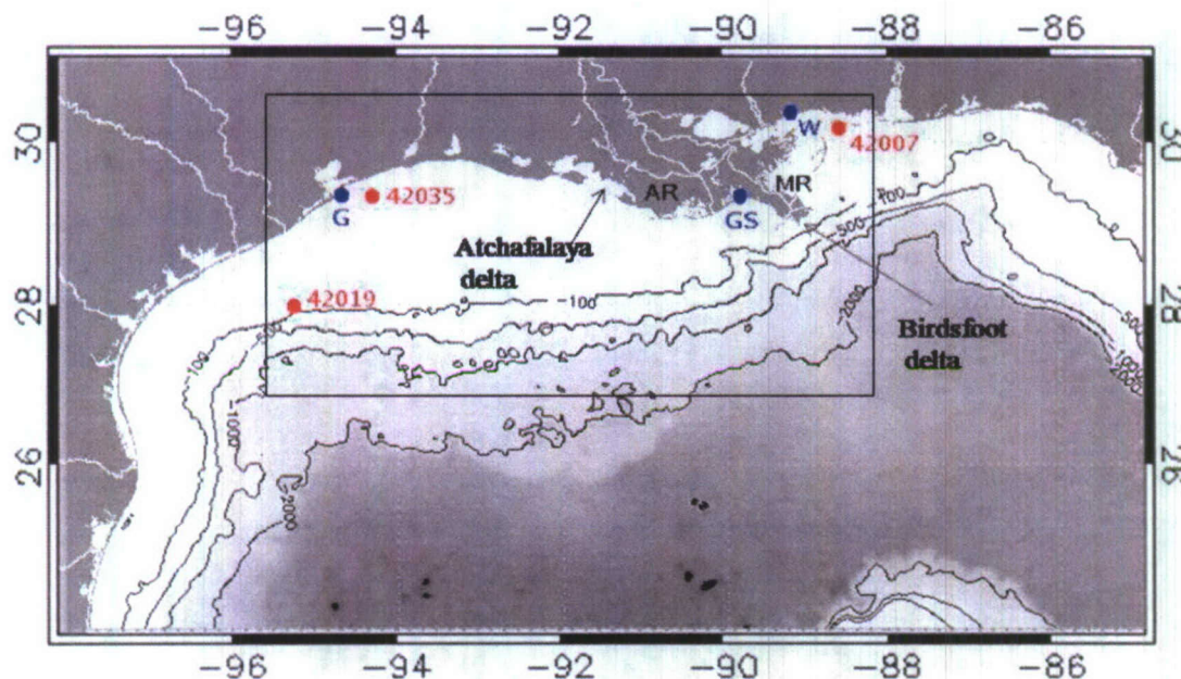
Figure 1. The study region in the northern Gulf of Mexico showing the domain (27–30.5°N latitude, 88.2–95.5°W longitude) of the nested coastal (MsLaTex) model and remote sensing data analysis (rectangular inset). The Mississippi River (MR) discharges through the birdsfoot delta while the Atchafalaya River (AR) lies to the west of MR. Smaller rivers and outlets include the Calcasieu, Sabine Lakes and the Trinity-San Jacinto estuary (G) located west of AR. The blue dots correspond to the location of three tide gauges located in Galveston (G)-Texas, Grand Isle (GS)-Louisiana and Waveland (W)-Mississippi. Also shown are the locations of three NOAA NDBC buoys within the study region.
