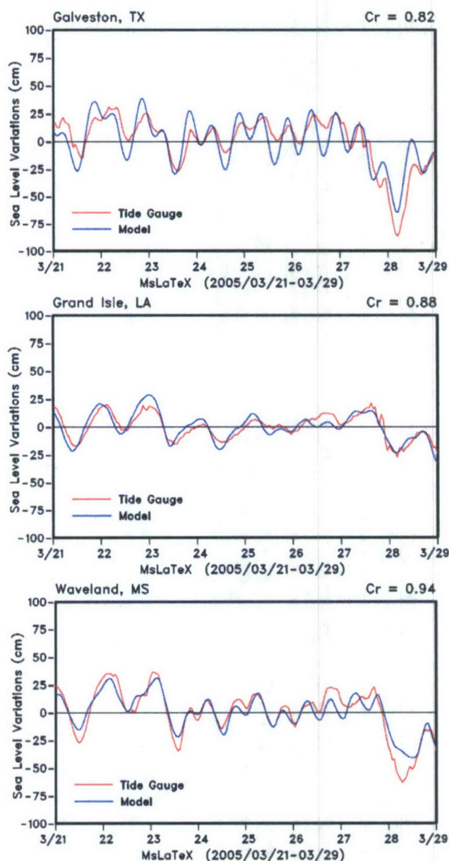
Figure 3. Sea level variations from model simulations (blue line) and tide gauge observations (red line) at (a) Galveston, Texas, (b) Grande Isle, Louisiana and (c) Waveland, Mississippi (shown in Fig. 1b) for the period 21-29 March 2005 corresponding to the frontal passages.
