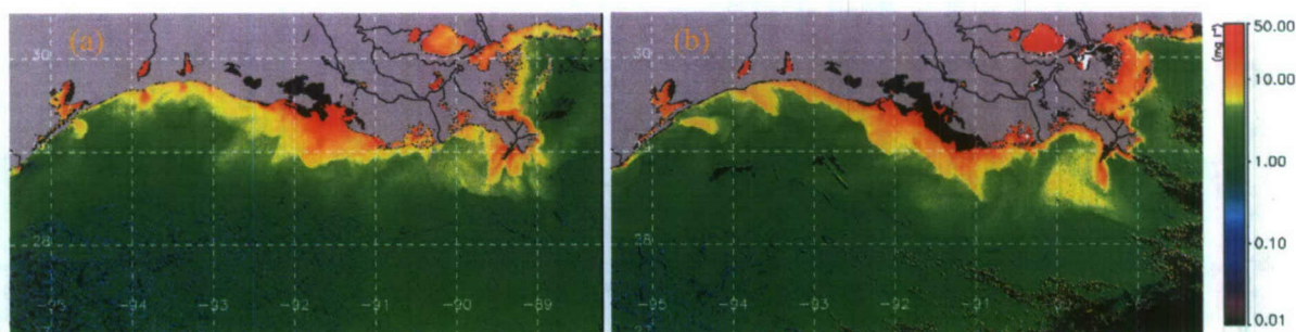
Figure 5. Suspended particulate matter (SPM) concentrations ( \text{mg l}^{-1} ) derived from SeaWiFS data for the study region on (a) 23 March and (b) 28 th March 2005. Clouds are masked to black.
