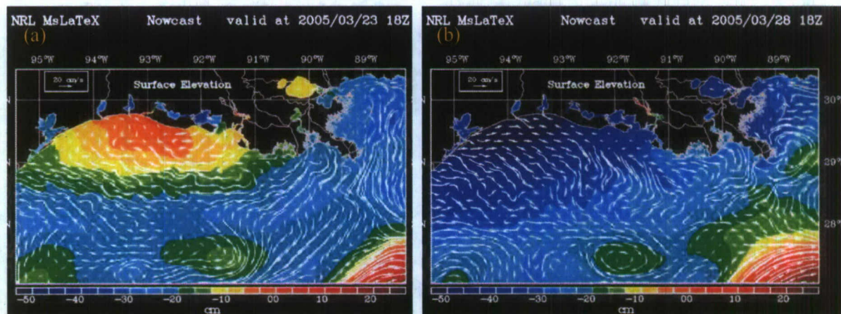
Figure 4. Model simulation of currents and surface elevation for 23 rd and 28 th March 2005. Current vectors are shown superimposed on the colored surface elevation map.
