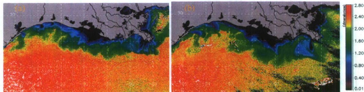
Figure 6. SeaWiFS derived imagery of spectral backscattering slope \gamma for (a) 23 March and (b) 28 March 2005.
