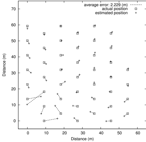
Figure 18: Centralized LSS localization results with the minimum spacing constraint. The average localization error is 2.2m.
