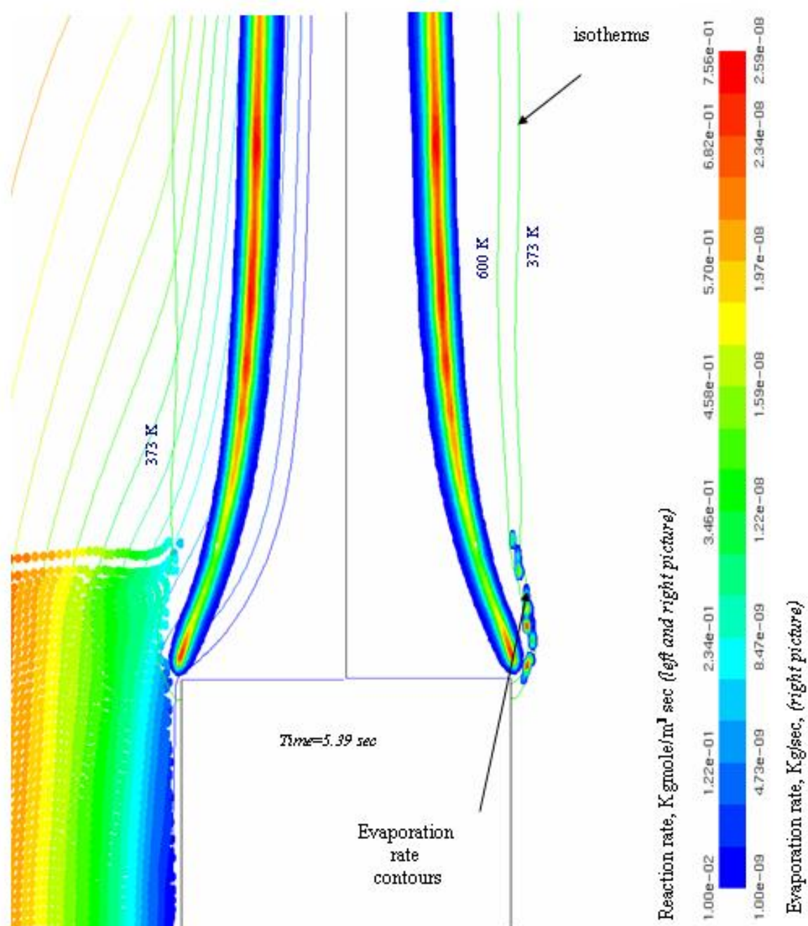
Figure 4b. Droplets evaporate between 373 and 600 K isotherms at 5.39 sec: 8 \mu\text{m} drops, 12 mass % total water. Left half of the burner : Droplet trajectories, gas streamlines (color lines), and 373 K isotherm (green line) superimposed on the reaction rate contours Right half of the burner : Evaporation rate contours superimposed on the reaction rate contours
