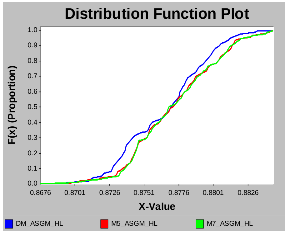
Figure 78 - ASGM Z_I CDF Comparison
