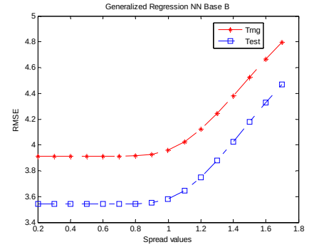
Figure 46 - Base B GRNN RMSE
