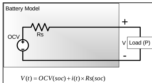
Figure 4-2 Battery Model
