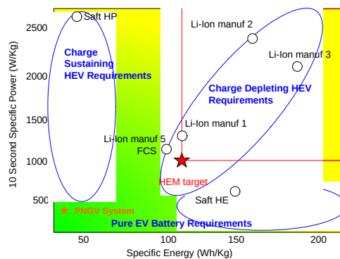
Figure 2-1 Energy and power requirements for different mode of operation
