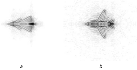
Fig. 2 Reference 256 \times 256 passive radar images reconstructed from ‘full’ datasets using direct Fourier reconstruction
