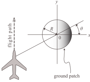
Fig. 5. Ground plane geometry in spotlight-mode SAR.
