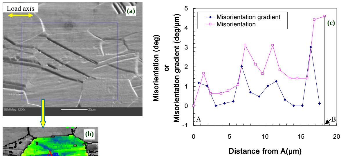
Fig. 3. (a) SEM image of an individual grain on the fully-recrystallized sample; (b) Misorientation map (rainbow scale: blue represents 0^\circ misorientation from reference and red represents 8^\circ misorientation from reference) with band contrasts and grain boundaries (black lines are high angle [ \theta > 10^\circ ] boundaries); (c) Misorientation angle and misorientation gradient profiles along a line from point A to point B shown in (b).
