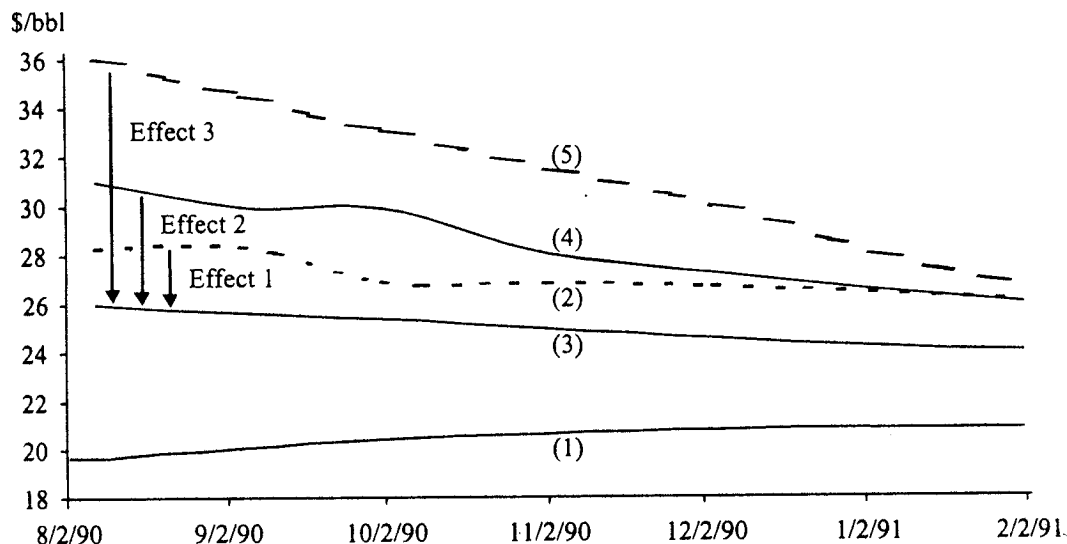
Figure 5: We used actual and hypothetical NYMEX oil-futures price curves to compute the economic benefits of naval crisis response. Curve 1 is the preinvasion futures prices for the next seven months (through the liberation of Kuwait). Curve 2 indicates the higher futures prices existing on August 7, 1990, five days after the invasion. Curve 3 indicates the reduction in futures prices found on August 9, 1990, after crisis response. Effect 1 measures the potential loss in gross domestic product that was avoided when futures prices shifted from Curve 2 to Curve 3 as a result of naval crisis response. For the US, Effect 1 was estimated to be worth $55.2 billion. Curve 4 is hypothetical in that it represents a possible futures prices curve had there been no crisis response. Effect 2 measures the potential loss in gross domestic product that would have resulted if there had been no crisis response, as indicated by the difference between Curve 4 and Curve 3. For the US, Effect 2 was estimated to be worth $94.0 billion. Curve 5 is a conservative estimate of what Curve 2 would have been if the invasion had occurred at a time of tight oil supplies. Effect 3 measures the potential loss in gross domestic product that would have resulted in such a scenario, as indicated by the difference between Curve 5 and Curve 3. For the US, Effect 3 was estimated to be worth $182.7 billion.
