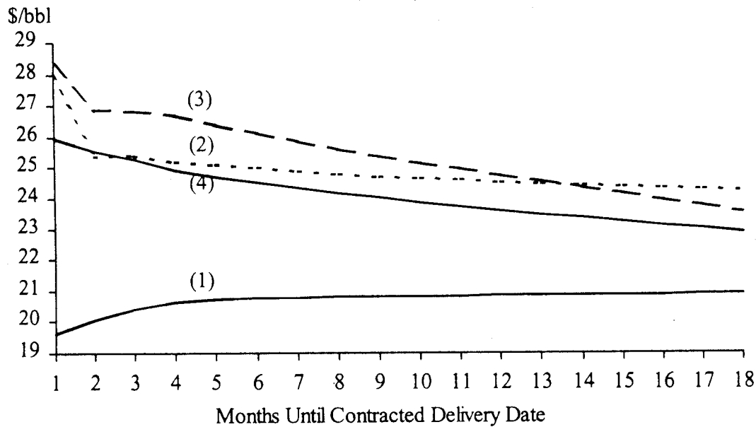
Figure 3: This figure is the Kuwait crisis realization of the notional behavior of NYMEX oil-futures prices shown in Figure 1. Curve 1 is the preinvasion price profile. Curve 2 is the postinvasion price profile of August 6, 1990, and Curve 3 is the postinvasion price profile of August 7, 1990. Curve 4 is the postinvasion price profile of August 8, 1990 as the market began to equilibrate. The invasion's impact on futures prices is clearly indicated by Curves 2 and 3: prices for all contract lengths increased and the slope of the curves is negative, indicating a willingness to pay a premium for immediate possession of oil. As evidenced by Curve 4, the impact of naval crisis response is a significant lowering of the entire futures price curve and a decrease in slope, reflecting the restoration of market confidence and reduced willingness to pay a premium for immediate possession of oil.
