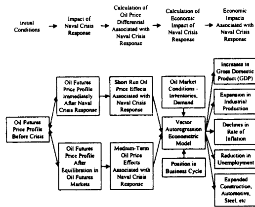
Figure 2: In our analysis, we tracked futures prices from prior to the crisis through the crisis and crisis response by naval forces. We used differences between the elevated futures prices created by the crisis and the futures prices moderated by crisis response to estimate the savings in oil purchased. We estimated the larger economic benefits of crisis response from an econometric model with these same oil price profiles. The econometric model indicates that naval crisis response prevents losses in economic activity.
