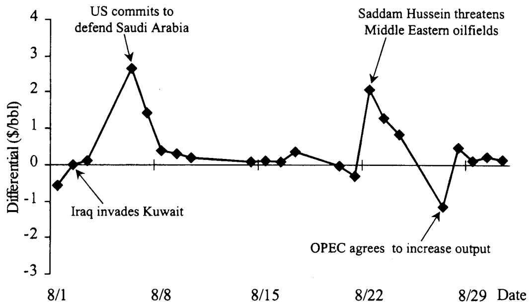
Figure 4: The NYMEX oil-futures prices show that when the differential between the first futures contract (September delivery) and the second futures contract (October delivery) is positive, traders prefer immediate possession of oil because they are concerned about its future availability. A return to equilibrium is indicated by the disappearance of a positive differential. An initial equilibrium is evidenced by the near-zero differential that exists between August 8, 1990 and August 22, 1990.
