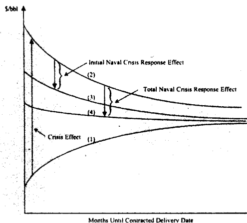
Figure 1: In the absence of a crisis, oil futures prices trend upward, reflecting, if nothing else, the cost of storing oil (Curve 1). A crisis in the region will cause a shock in prices, illustrated by the upward shift and change in slope from Curve 1 to Curve 2, reflecting traders' willingness to pay a premium for the immediate possession of oil due to concern about its future availability. Crisis response by naval forces moderates concerns about future availability of oil and lowers the futures price curve over all contract periods (Curve 3). This trend continues until market confidence is restored and the markets equilibrate (Curve 4).
