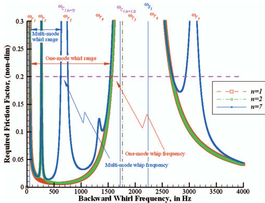
Figure 5 Multi-mode dry-friction whirl prediction for Bartha's test rig [5]
