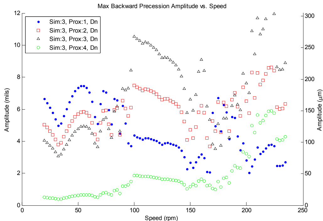
Figure 30 Predicted backward precession amplitude versus speed for all probes
