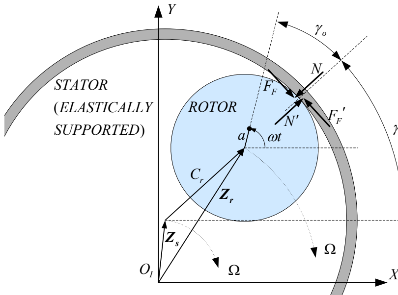
Figure 2 Rotor-stator interaction model, after [5]
