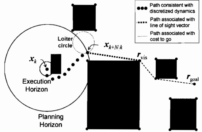
Fig. 1. Representation of the cost-to-go function showing the three levels of resolution used to approximate a complete path to the goal.
