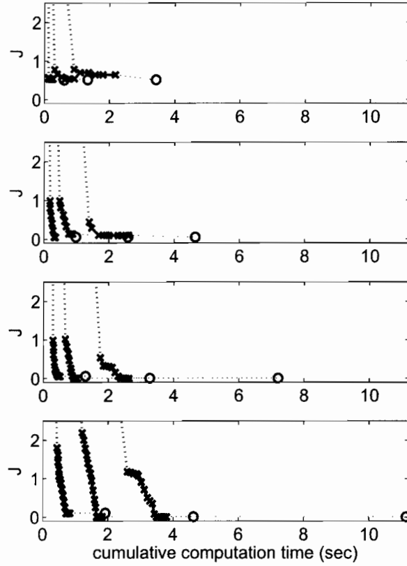
Fig. 9. Trade-off between the performance and the computation time. From the top to the bottom, the number of vehicles are 5, 7, 10, and 15.
