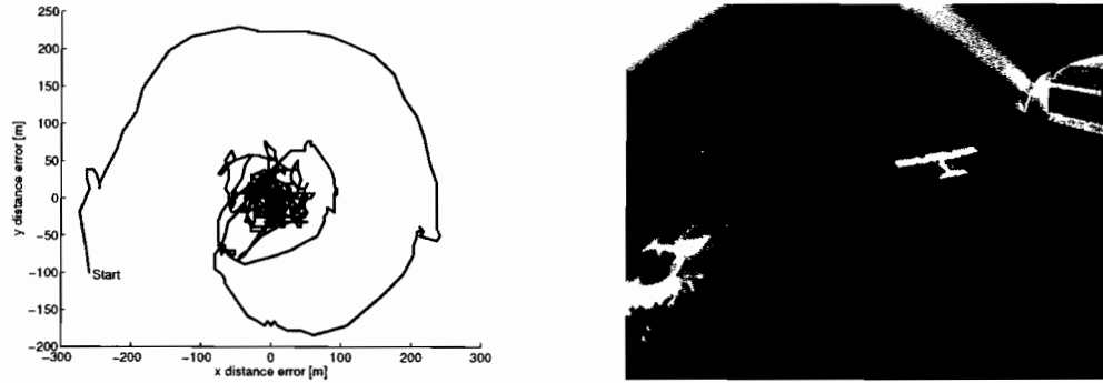
Fig. 4: Flight data showing show the relative separation error between 2 UAVs during an autonomous in-flight rendezvous with a photo from onboard.
