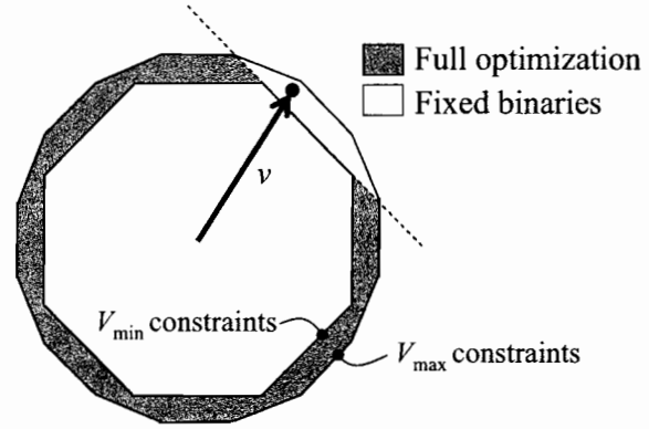
Fig. 4. Feasible perturbation of the velocity, with fixed v_{\min} binaries
