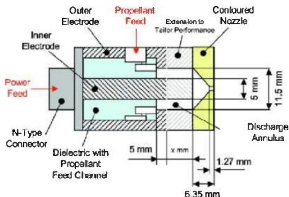
FIGURE 1. Schematic of the experimental RF plasma thruster.
