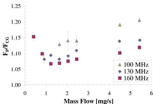
FIGURE 9. Thrust ratio as a function of \dot{m} and frequency.
