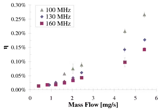
FIGURE 11. Propulsive efficiency as a function of \dot{m} and frequency.
