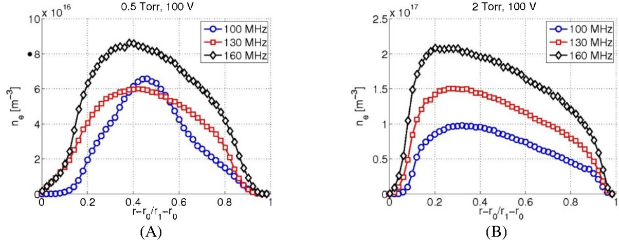
FIGURE 3: Calculated electron number density for V=100 Volts. (A) P_0=0.5 Torr, (B) P_0=2.0 Torr.
