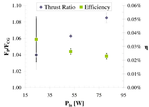
FIGURE 8. Thrust ratio and efficiency as a function of input power.
