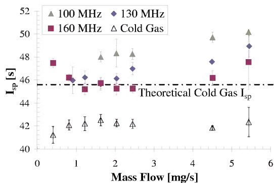
FIGURE 10. Specific impulse as a function of \dot{m} and frequency.
