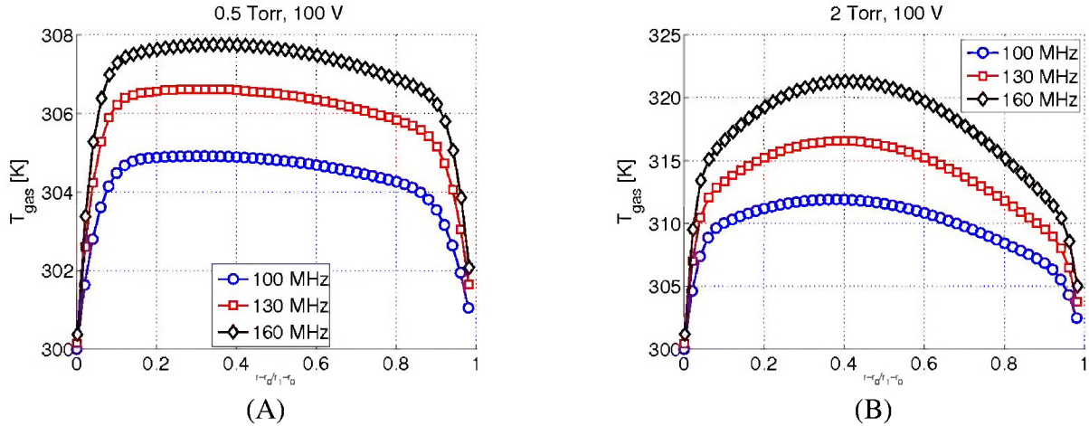
FIGURE 4: Calculated neutral gas temperature for V=100 Volts. (A) P_0=0.5 Torr, (B) P_0=2.0 Torr.
