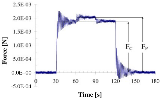
FIGURE 7. A typical powered trace from the nNTS.
