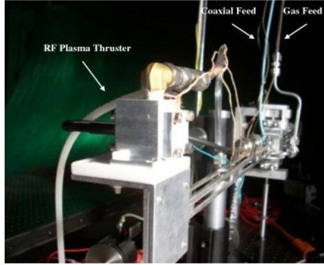
FIGURE 6. The RF Plasma thruster attached to the arm of the nNTS. The electrostatic comb calibration system was attached to the opposite arm of the thrust stand.
