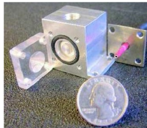
FIGURE 2. Experimental RFCCD.
