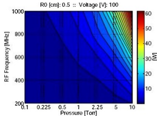
FIGURE 5. Power transmitted to propellant as a function of discharge pressure and applied frequency.
