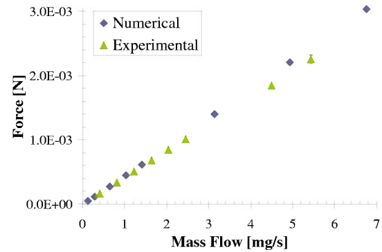
FIGURE 12. Cold gas thrust as a function of \dot{m} .
