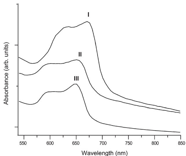
Fig. 4 Visible absorption spectra for I , II , and III showing two absorption maxima for each material at: I = 664, 622 nm; II = 646, 602 nm and III = 643, 596 nm.
