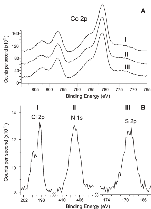
Fig. 3 High resolution XPS spectra of (A) Co 2p region for I , II , and III and (B) Cl 2p, N 1s and S 2p regions for I , II , and III respectively.
