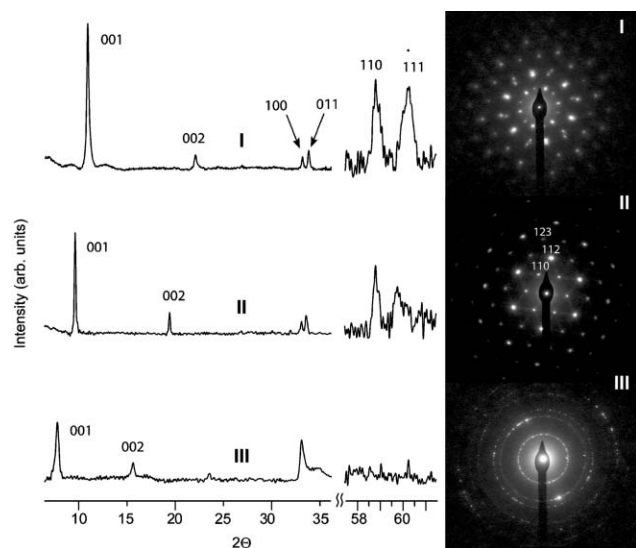
Fig. 2 Powder XRD and electron diffraction patterns for I , II , and III showing peaks indexing to the hydrotalcite-like structure with a_{\text{I,II,III}} = 3.13 \text{ \AA} ; c_{\text{I}} = 8.12 \text{ \AA} ; c_{\text{II}} = 9.19 \text{ \AA} ; and c_{\text{III}} = 11.26 \text{ \AA} . Electron diffraction patterns showing only II is single crystalline whereas I and III exhibit varying degrees of polycrystallinity. XRD spectra are magnified by 10\times after the break in 2\theta . Electron diffraction index labels belong to the spots immediately below the text.
