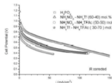
Fig.2: H_2/O_2 fuel cell using ETEK electrodes (Pt 0.5 mg/cm²) with binary mixtures and 85% aqueous H_3PO_4 as the electrolyte at 140°C. (From Ref. 12, by permission).
