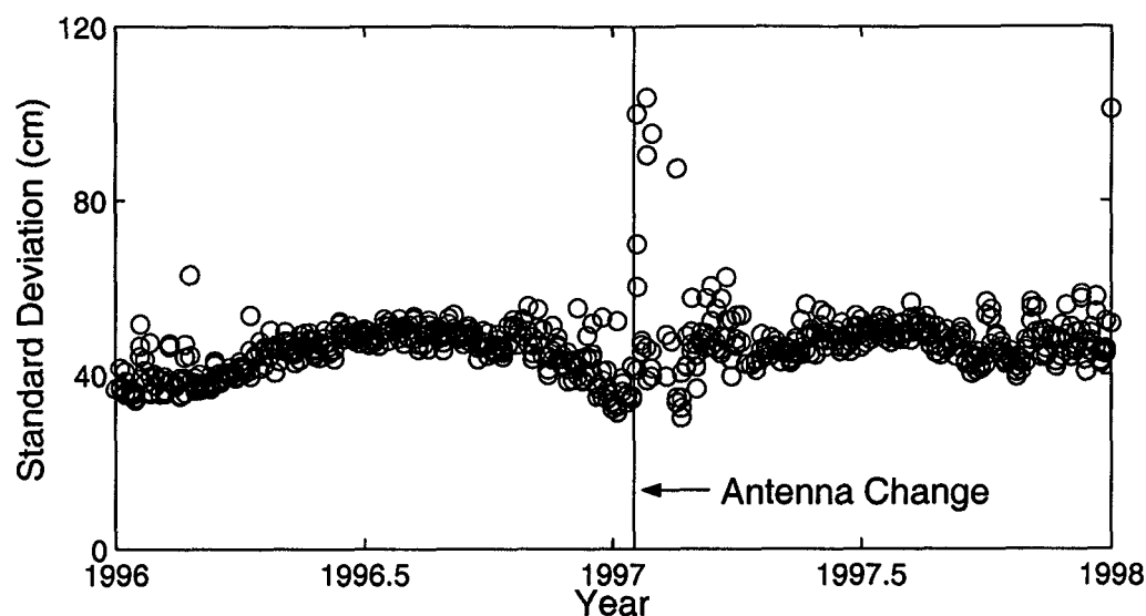
Figure 9: Standard deviation of P3 postfit residuals at ALGO from 1996-1998. Note the immediate increase in number and magnitude of outliers once the antenna was replaced in January 1997. The broad seasonal variation in the standard deviation has not been modeled, but was significantly reduced by the installation of a new receiver in 1999.
