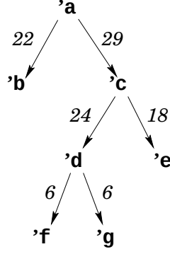
Figure 3: The multicast distribution tree corresponding to RTTstate2 .
