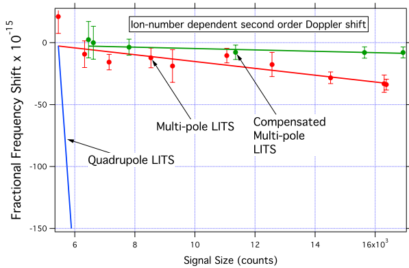
Figure 10. The ion-number-dependent second order Doppler shift for the quadrupole LITS (blue), the multi-pole LITS operating with AUX1 set to produce the most uniform field (red) and the multi-pole LITS operating with AUX1 set to produce optimal cancellation of the number-dependent effect (green). The total fractional frequency shift is about 3 \times 10^{-12} for the quadrupole LITS, 3 \times 10^{-14} for the multi-pole LITS and < 5 \times 10^{-15} for the "compensated" multi-pole LITS.
