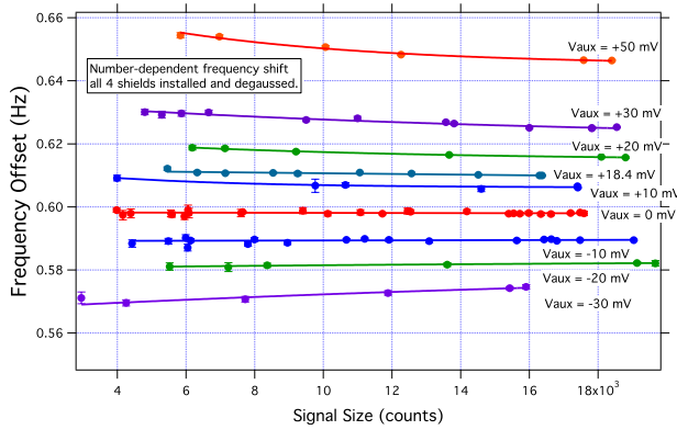
Figure 8. Measured LITS-9 frequency shifts after the magnetic shields have been degaussed. All shifts are relative to the 40.5 GHz \text{Hg}^+ clock transition frequency. The picture remains qualitatively the same, but a different overall offset is introduced.
