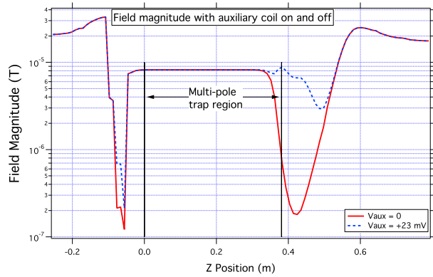
Figure 4. A plot of the modeled magnetic field magnitude along the axis of the LITS-9 physics package. The solid red line shows the field with only the C-field on. The dashed blue line shows that field modified by the application of the auxiliary coil at the interface between the quadrupole and multi-pole traps, which is also at one end of the C-field solenoid (AUX1). The axial position of 0 m corresponds to the lower end of the C-field solenoid (left side as viewed in the figure) and the region between the vertical black lines corresponds to the multi-pole trap.
