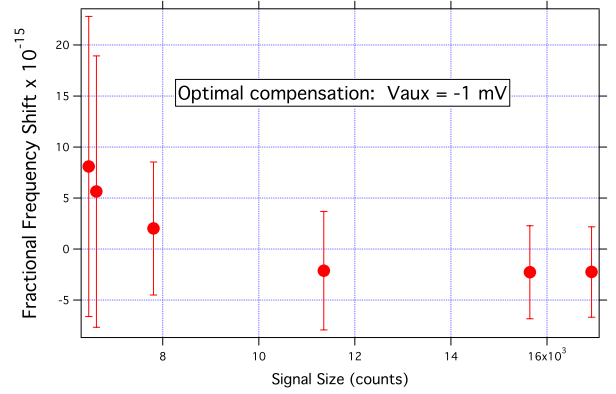
Figure 9. Frequency shift vs. ion number (signal size) data for the optimal AUX1 coil setting (minimal ion-number dependence). Each data point represents 6 hours of data with the error bars representing 3- \sigma statistical errors.
